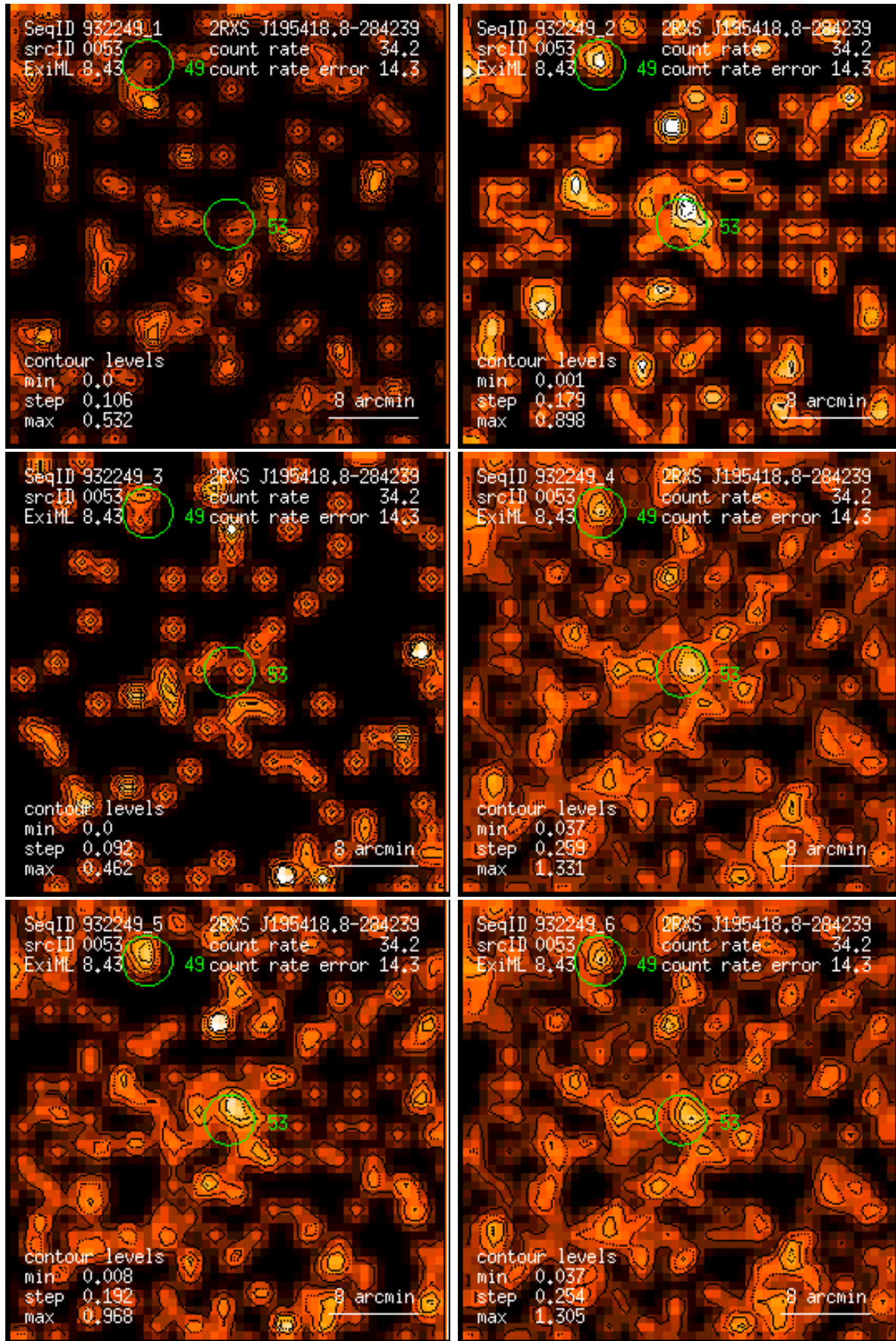
Figure 53: RASS 932249: detection 0053: band rate images, Gaussian filter: (1) PSPC channels 11 – 41, (2) 52 – 90, (3) 91 – 201, (4) 11 – 235, (5) 52 – 201, (6) 11 – 201. Broad band rates in counts/ks. Band rate contour levels in counts/ks/arcmin 2 .
