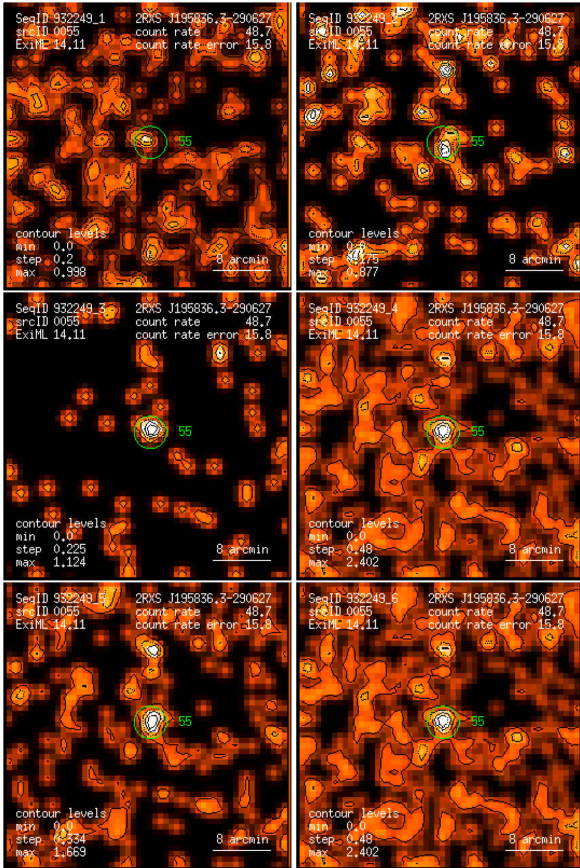
Figure 55: RASS 932249: detection 0055: band rate images, Gaussian filter: (1) PSPC channels 11 – 41, (2) 52 – 90, (3) 91 – 201, (4) 11 – 235, (5) 52 – 201, (6) 11 – 201. Broad band rates in counts/ks. Band rate contour levels in counts/ks/arcmin 2 .
