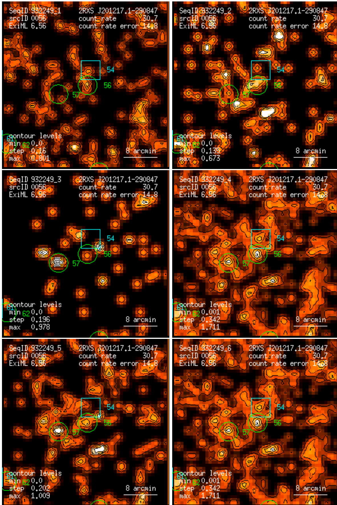
Figure 56: RASS 932249: detection 0056: band rate images, Gaussian filter: (1) PSPC channels 11 – 41, (2) 52 – 90, (3) 91 – 201, (4) 11 – 235, (5) 52 – 201, (6) 11 – 201. Broad band rates in counts/ks. Band rate contour levels in counts/ks/arcmin 2 .
