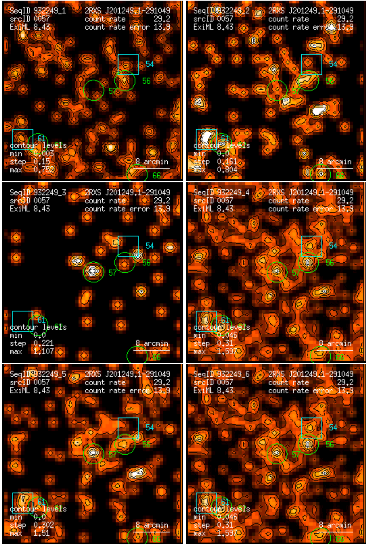
Figure 57: RASS 932249: detection 0057: band rate images, Gaussian filter: (1) PSPC channels 11 – 41, (2) 52 – 90, (3) 91 – 201, (4) 11 – 235, (5) 52 – 201, (6) 11 – 201. Broad band rates in counts/ks. Band rate contour levels in counts/ks/arcmin 2 .
