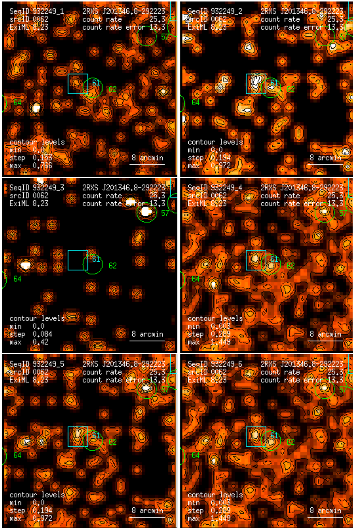
Figure 62: RASS 932249: detection 0062: band rate images, Gaussian filter: (1) PSPC channels 11 – 41, (2) 52 – 90, (3) 91 – 201, (4) 11 – 235, (5) 52 – 201, (6) 11 – 201. Broad band rates in counts/ks. Band rate contour levels in counts/ks/arcmin 2 .
