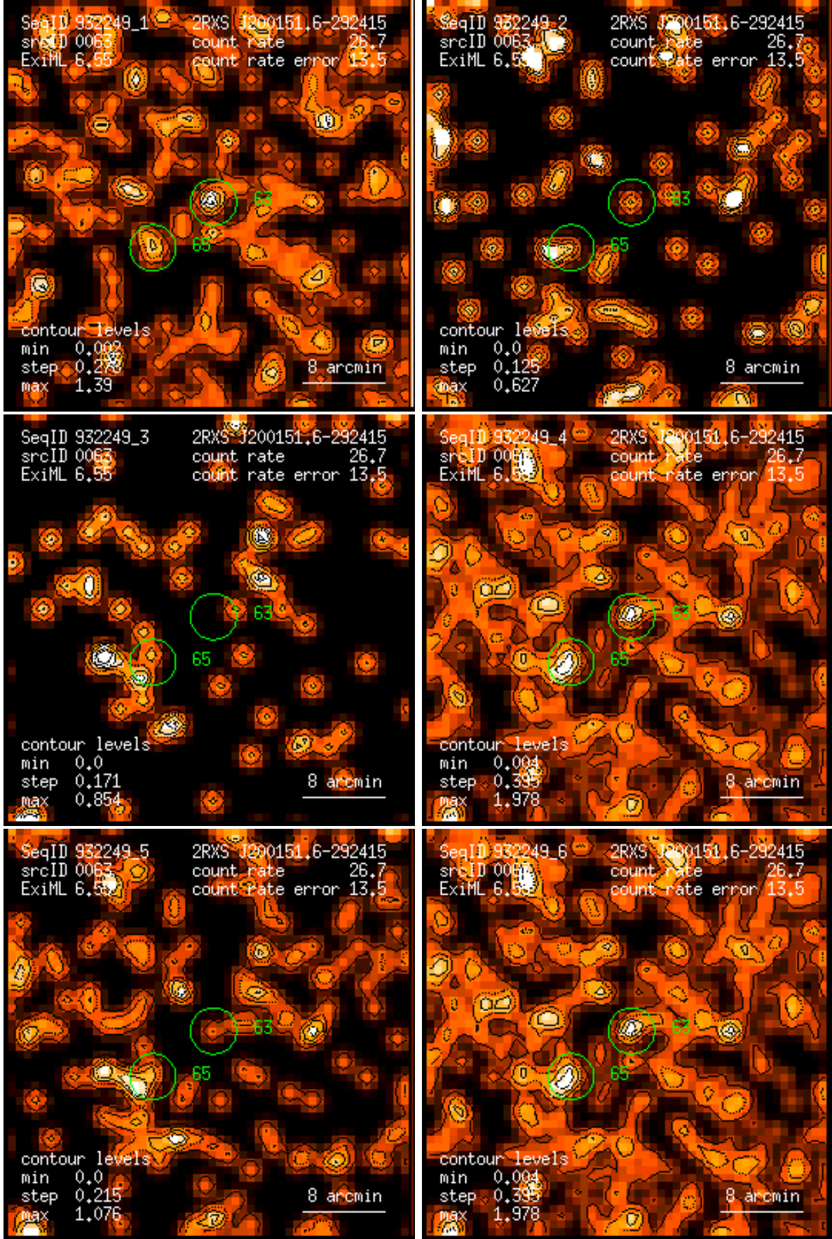
Figure 63: RASS 932249: detection 0063: band rate images, Gaussian filter: (1) PSPC channels 11 – 41, (2) 52 – 90, (3) 91 – 201, (4) 11 – 235, (5) 52 – 201, (6) 11 – 201. Broad band rates in counts/ks. Band rate contour levels in counts/ks/arcmin 2 .
