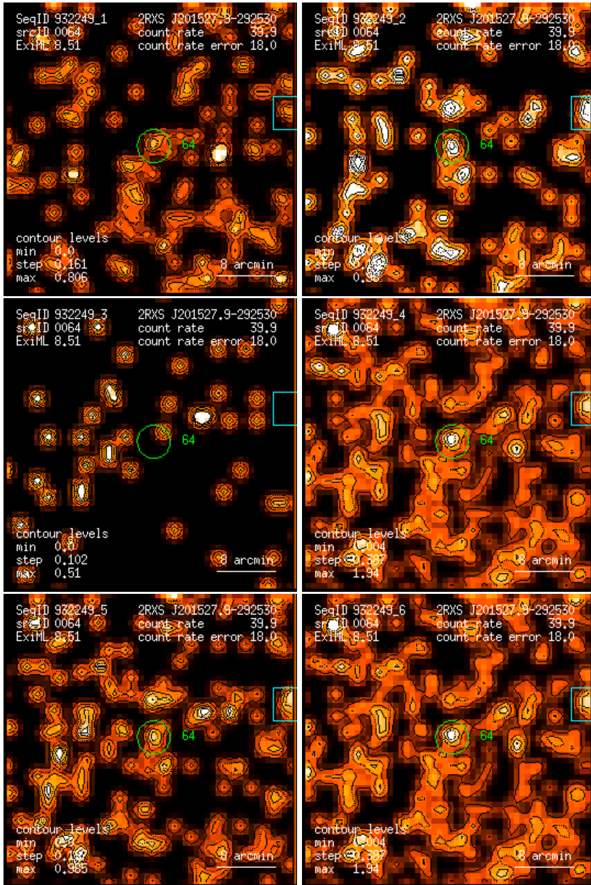
Figure 64: RASS 932249: detection 0064: band rate images, Gaussian filter: (1) PSPC channels 11 – 41, (2) 52 – 90, (3) 91 – 201, (4) 11 – 235, (5) 52 – 201, (6) 11 – 201. Broad band rates in counts/ks. Band rate contour levels in counts/ks/arcmin 2 .
