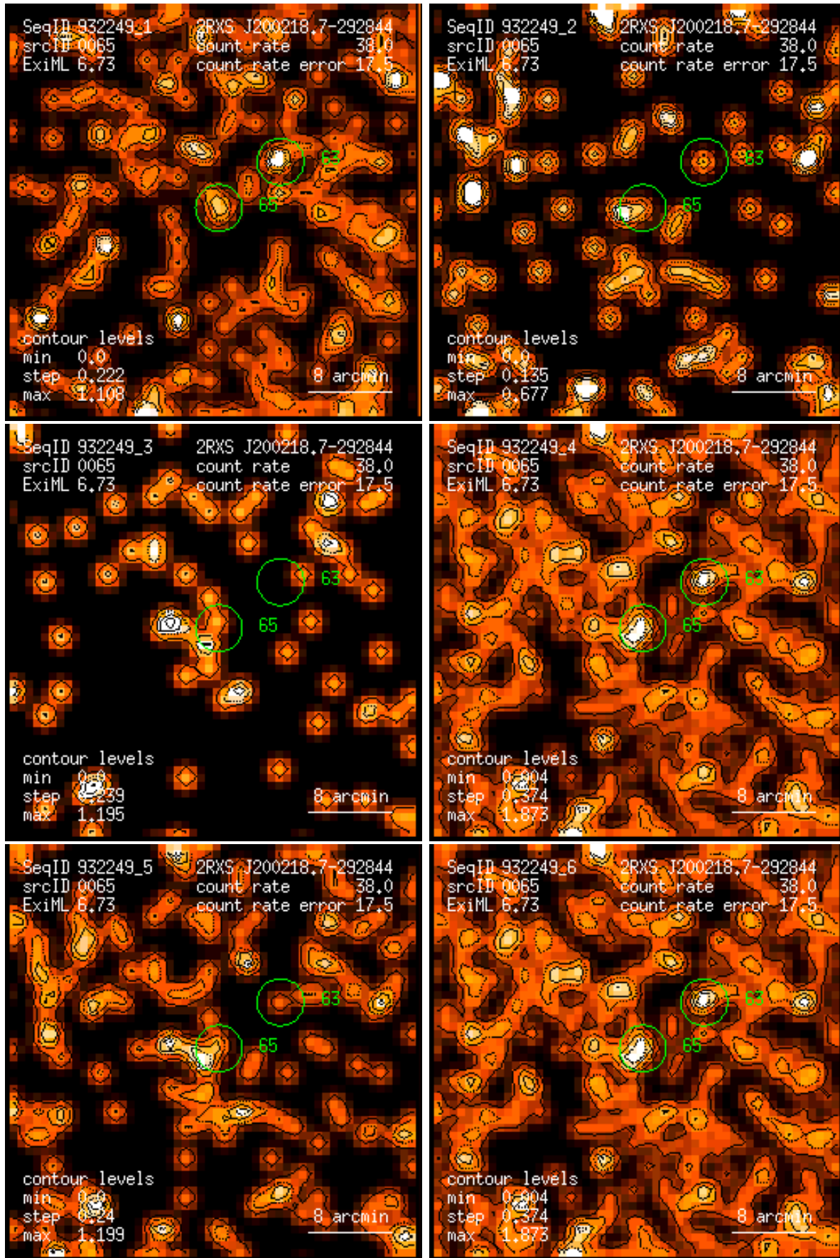
Figure 65: RASS 932249: detection 0065: band rate images, Gaussian filter: (1) PSPC channels 11 – 41, (2) 52 – 90, (3) 91 – 201, (4) 11 – 235, (5) 52 – 201, (6) 11 – 201. Broad band rates in counts/ks. Band rate contour levels in counts/ks/arcmin 2 .
