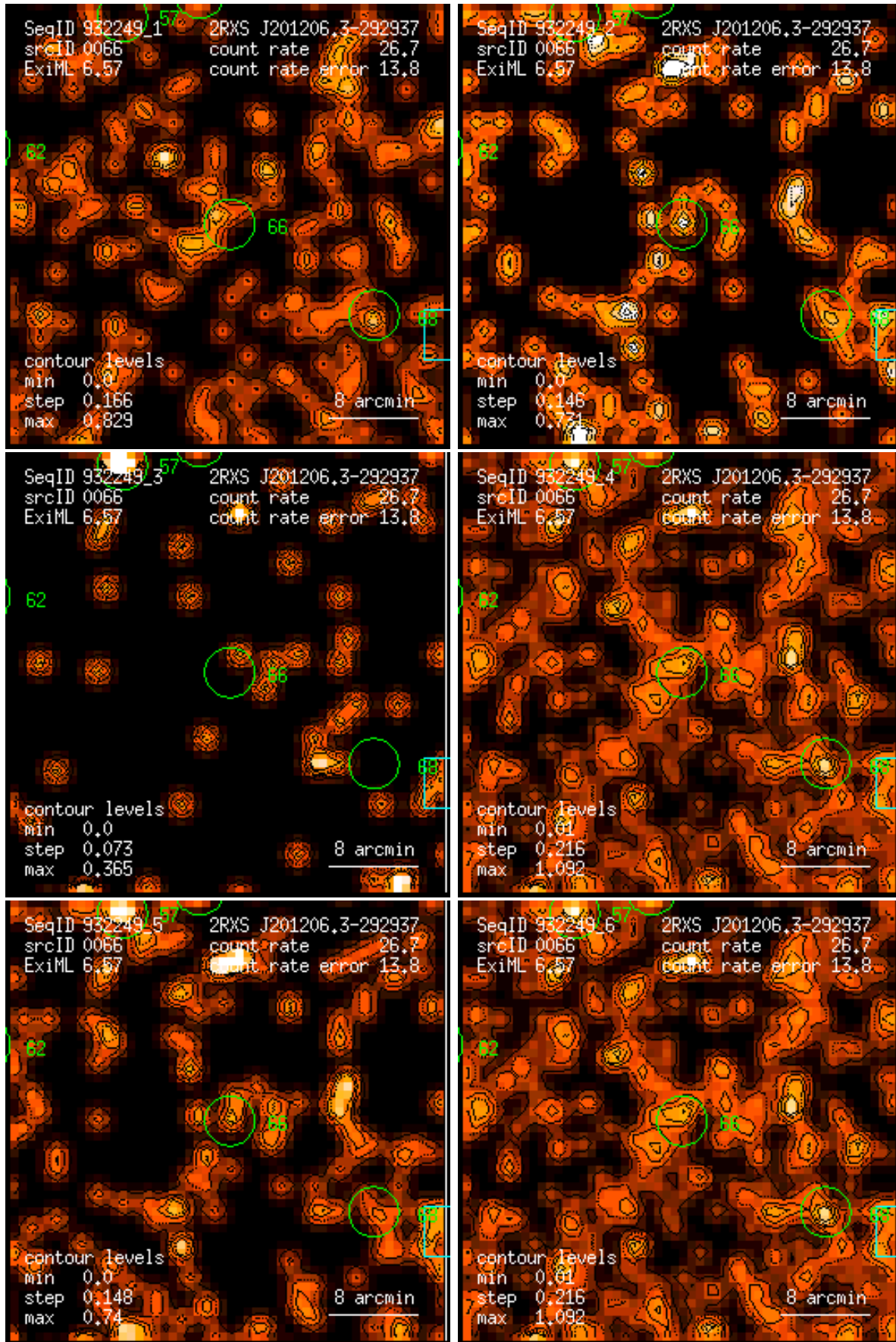
Figure 66: RASS 932249: detection 0066: band rate images, Gaussian filter: (1) PSPC channels 11 – 41, (2) 52 – 90, (3) 91 – 201, (4) 11 – 235, (5) 52 – 201, (6) 11 – 201. Broad band rates in counts/ks. Band rate contour levels in counts/ks/arcmin 2 .
