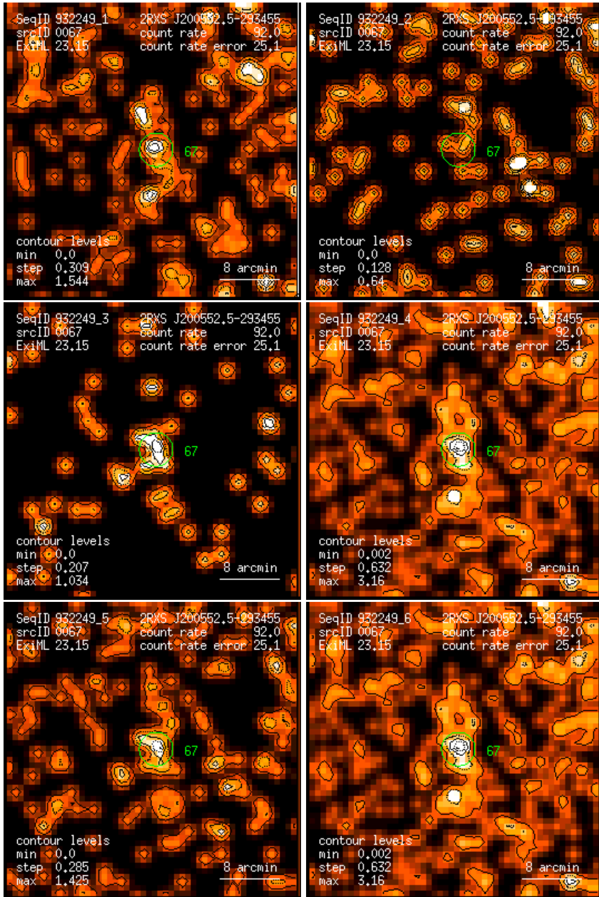
Figure 67: RASS 932249: detection 0067: band rate images, Gaussian filter: (1) PSPC channels 11 – 41, (2) 52 – 90, (3) 91 – 201, (4) 11 – 235, (5) 52 – 201, (6) 11 – 201. Broad band rates in counts/ks. Band rate contour levels in counts/ks/arcmin 2 .
