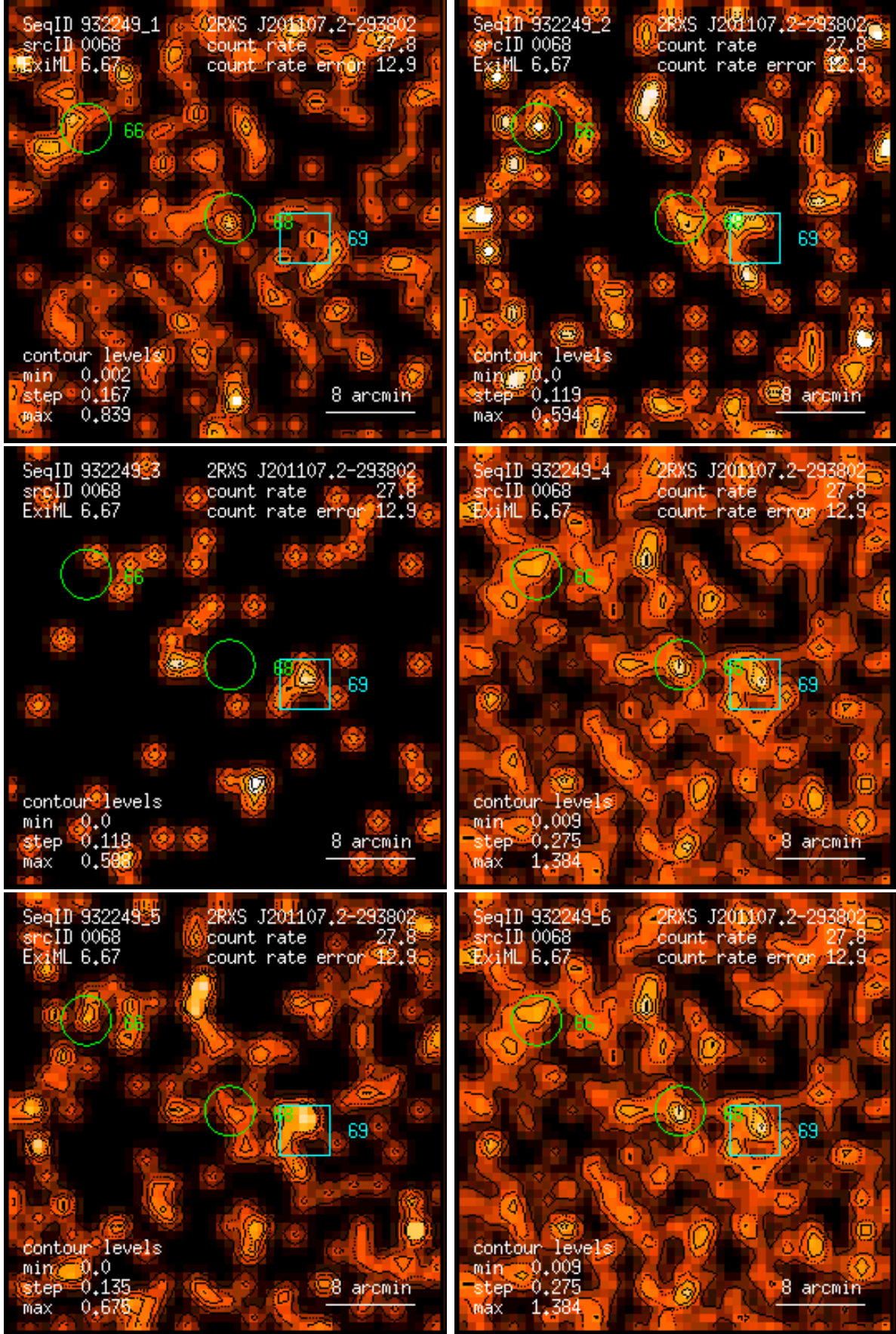
Figure 68: RASS 932249: detection 0068: band rate images, Gaussian filter: (1) PSPC channels 11 – 41, (2) 52 – 90, (3) 91 – 201, (4) 11 – 235, (5) 52 – 201, (6) 11 – 201. Broad band rates in counts/ks. Band rate contour levels in counts/ks/arcmin 2 .
