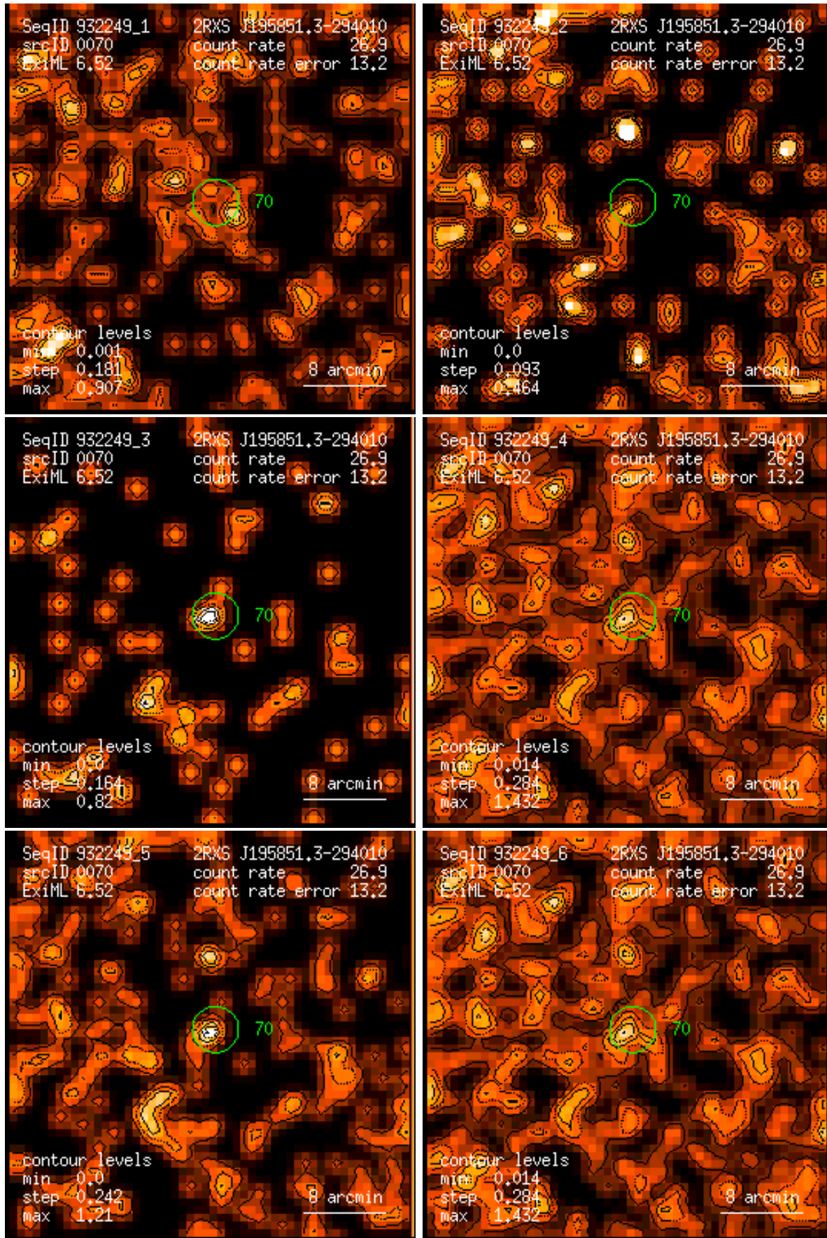
Figure 70: RASS 932249: detection 0070: band rate images, Gaussian filter: (1) PSPC channels 11 – 41, (2) 52 – 90, (3) 91 – 201, (4) 11 – 235, (5) 52 – 201, (6) 11 – 201. Broad band rates in counts/ks. Band rate contour levels in counts/ks/arcmin 2 .
