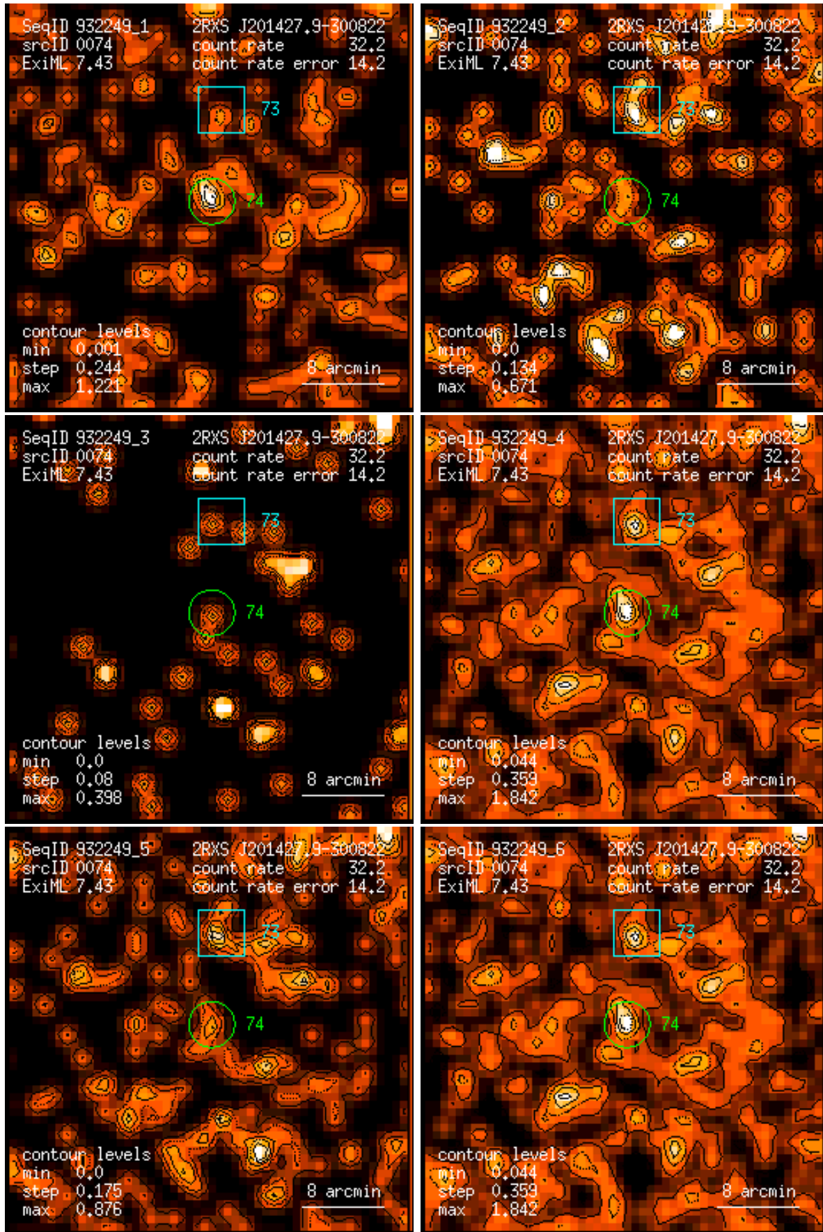
Figure 74: RASS 932249: detection 0074: band rate images, Gaussian filter: (1) PSPC channels 11 – 41, (2) 52 – 90, (3) 91 – 201, (4) 11 – 235, (5) 52 – 201, (6) 11 – 201. Broad band rates in counts/ks. Band rate contour levels in counts/ks/arcmin 2 .
