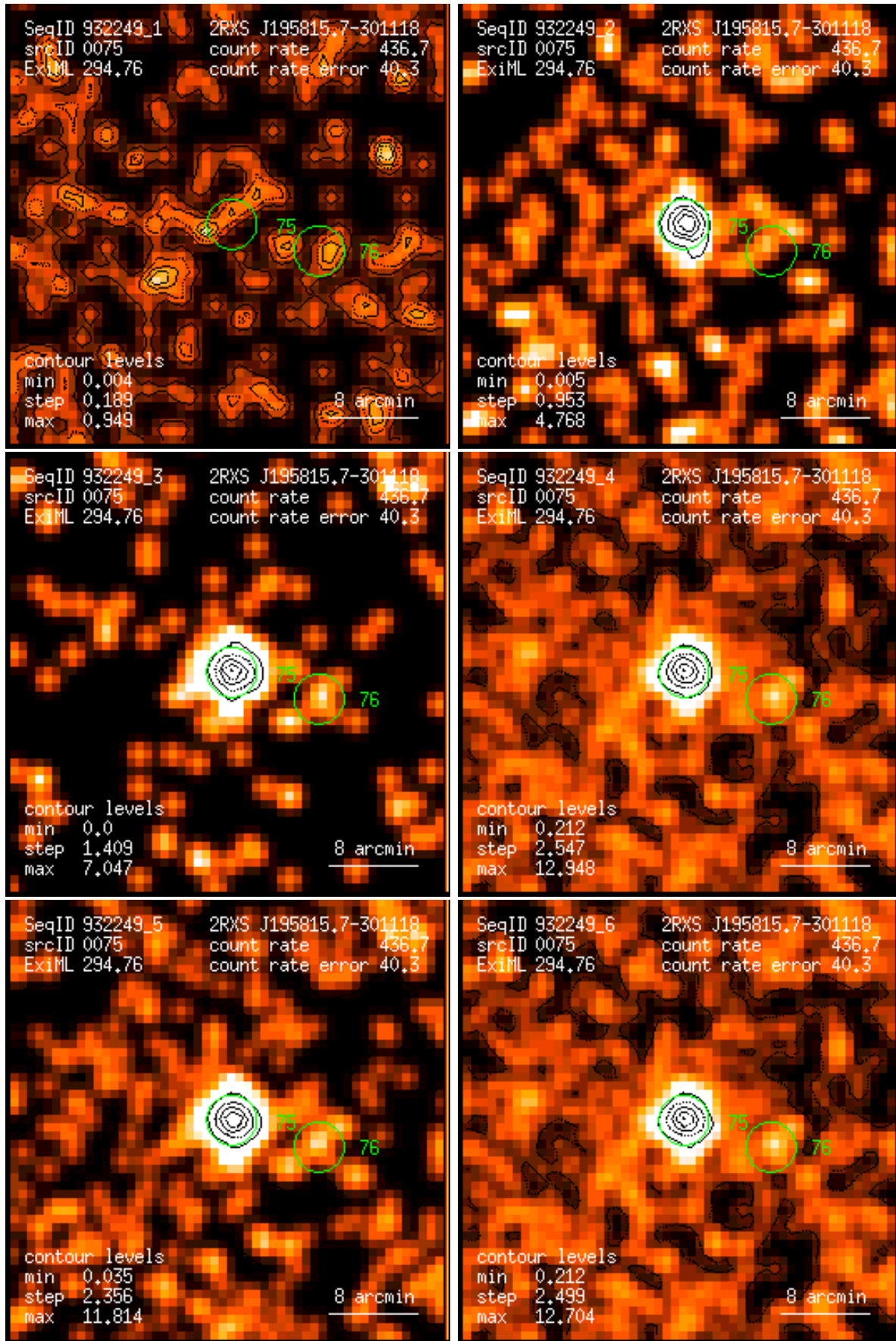
Figure 75: RASS 932249: detection 0075: band rate images, Gaussian filter: (1) PSPC channels 11 – 41, (2) 52 – 90, (3) 91 – 201, (4) 11 – 235, (5) 52 – 201, (6) 11 – 201. Broad band rates in counts/ks. Band rate contour levels in counts/ks/arcmin 2 .
