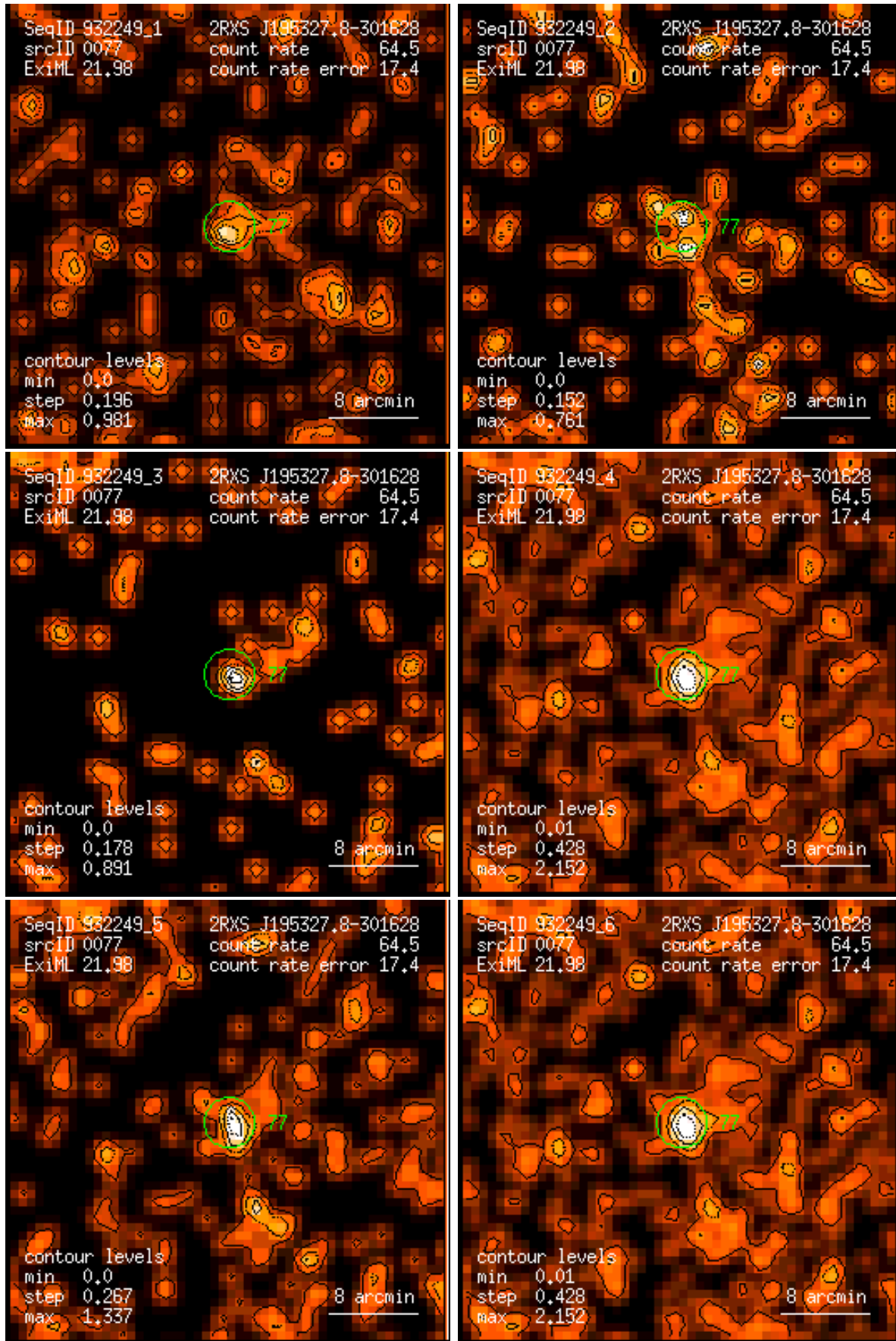
Figure 77: RASS 932249: detection 0077: band rate images, Gaussian filter: (1) PSPC channels 11 – 41, (2) 52 – 90, (3) 91 – 201, (4) 11 – 235, (5) 52 – 201, (6) 11 – 201. Broad band rates in counts/ks. Band rate contour levels in counts/ks/arcmin 2 .
