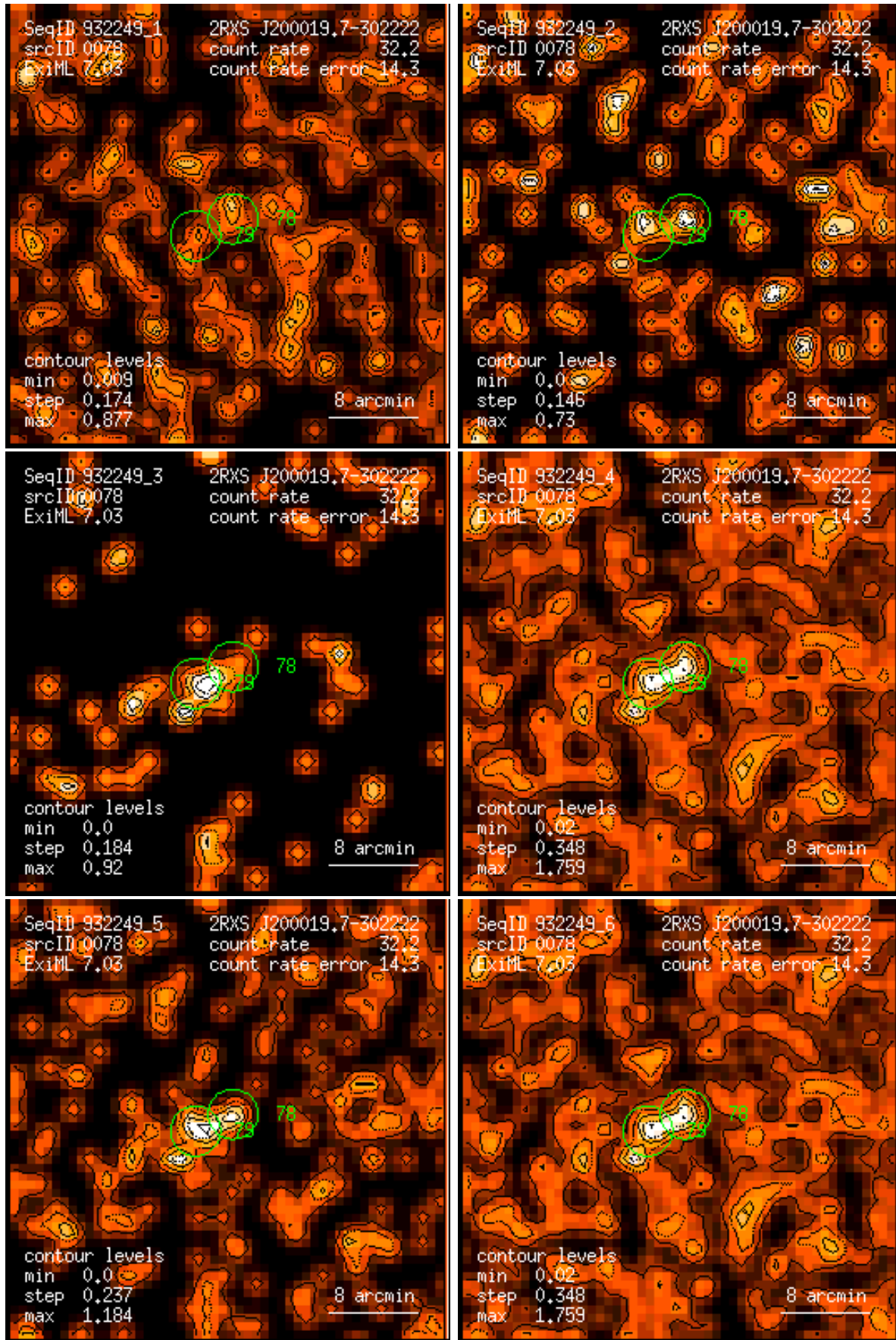
Figure 78: RASS 932249: detection 0078: band rate images, Gaussian filter: (1) PSPC channels 11 – 41, (2) 52 – 90, (3) 91 – 201, (4) 11 – 235, (5) 52 – 201, (6) 11 – 201. Broad band rates in counts/ks. Band rate contour levels in counts/ks/arcmin 2 .
