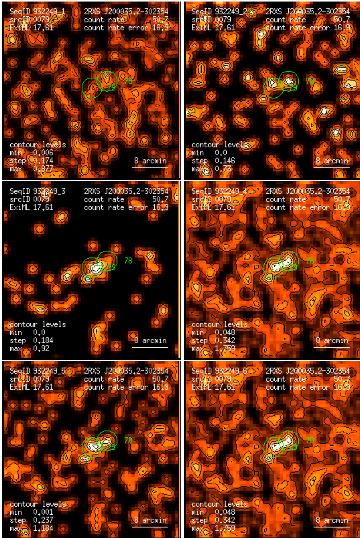
Figure 79: RASS 932249: detection 0079: band rate images, Gaussian filter: (1) PSPC channels 11 – 41, (2) 52 – 90, (3) 91 – 201, (4) 11 – 235, (5) 52 – 201, (6) 11 – 201. Broad band rates in counts/ks. Band rate contour levels in counts/ks/arcmin 2 .
