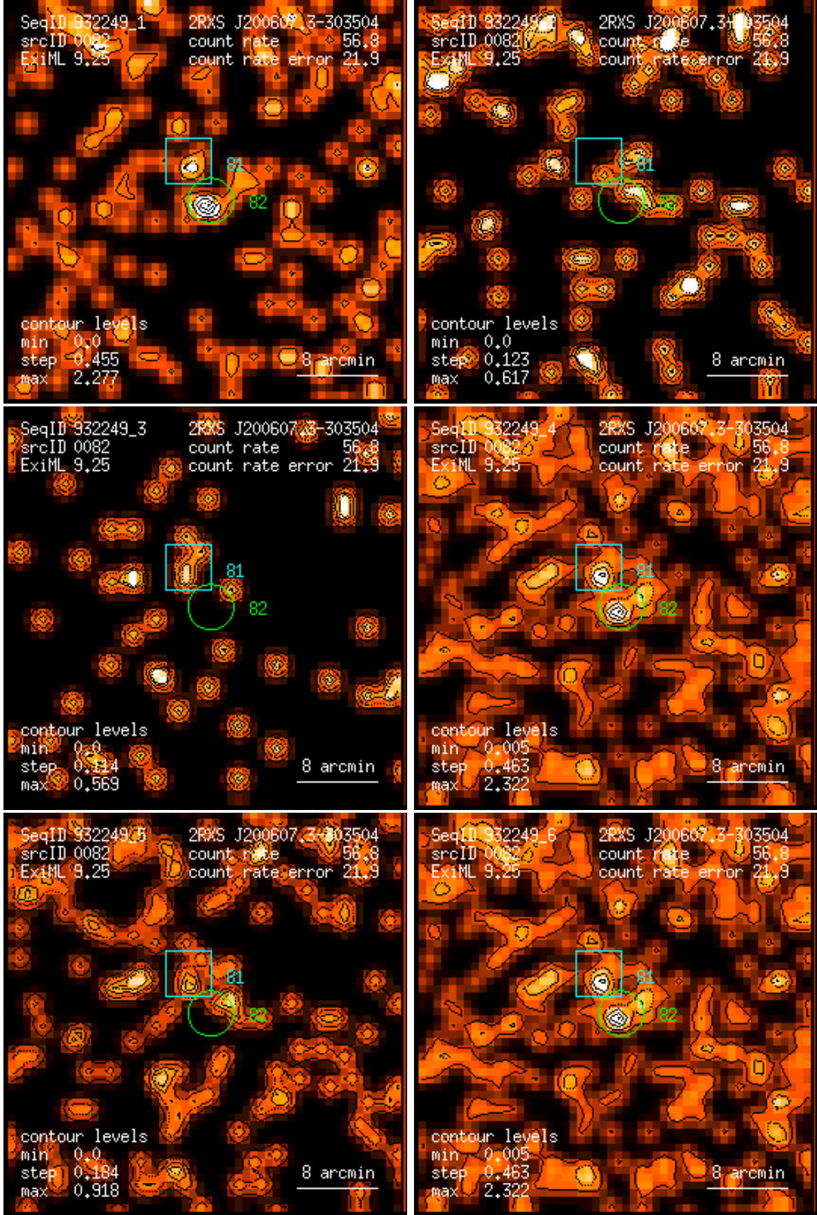
Figure 82: RASS 932249: detection 0082: band rate images, Gaussian filter: (1) PSPC channels 11 – 41, (2) 52 – 90, (3) 91 – 201, (4) 11 – 235, (5) 52 – 201, (6) 11 – 201. Broad band rates in counts/ks. Band rate contour levels in counts/ks/arcmin 2 .
