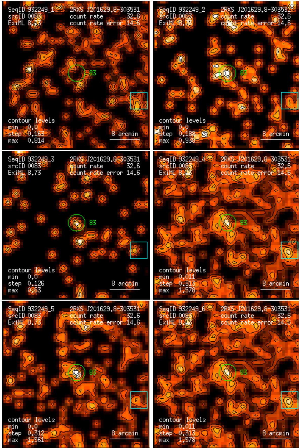
Figure 83: RASS 932249: detection 0083: band rate images, Gaussian filter: (1) PSPC channels 11 – 41, (2) 52 – 90, (3) 91 – 201, (4) 11 – 235, (5) 52 – 201, (6) 11 – 201. Broad band rates in counts/ks. Band rate contour levels in counts/ks/arcmin 2 .
