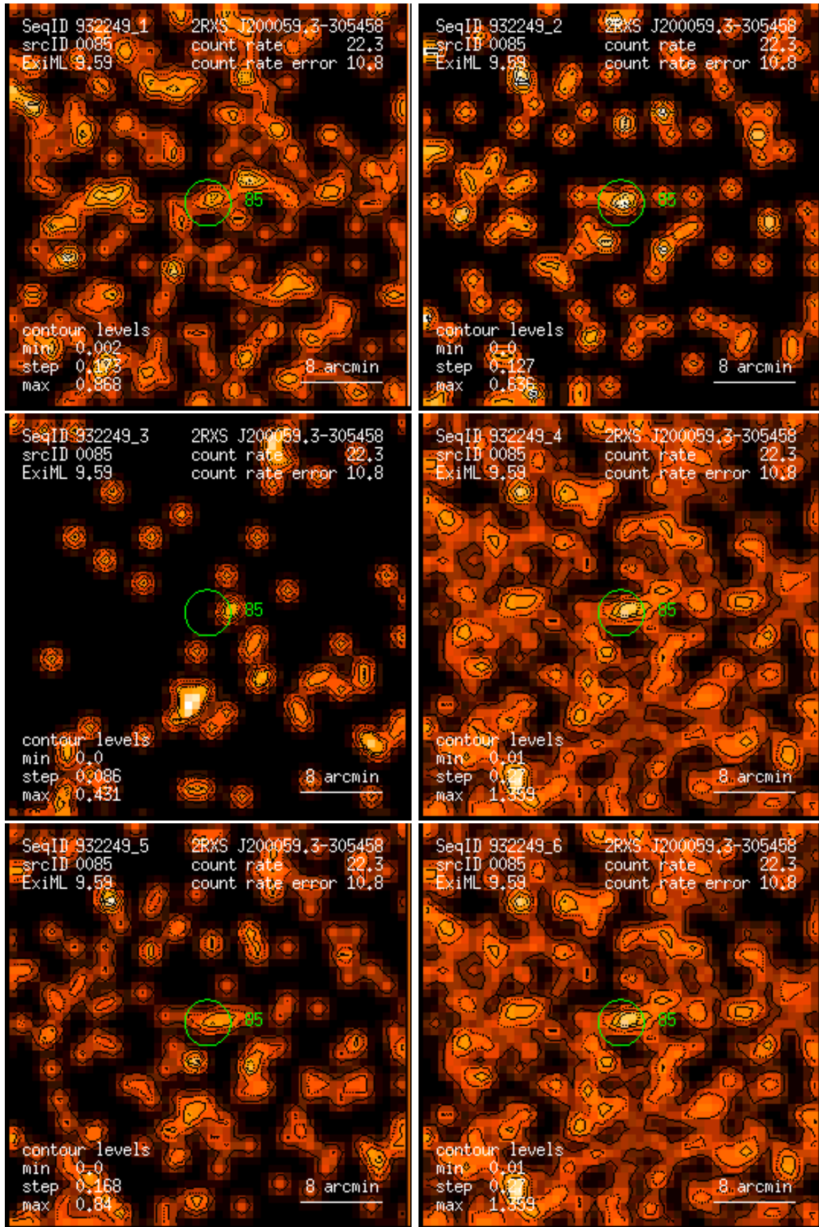
Figure 85: RASS 932249: detection 0085: band rate images, Gaussian filter: (1) PSPC channels 11 – 41, (2) 52 – 90, (3) 91 – 201, (4) 11 – 235, (5) 52 – 201, (6) 11 – 201. Broad band rates in counts/ks. Band rate contour levels in counts/ks/arcmin 2 .
