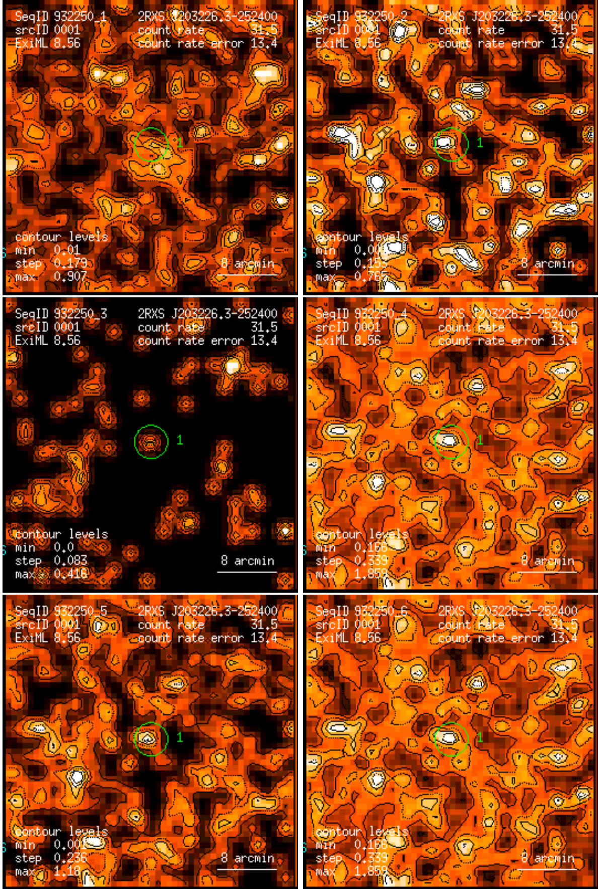
Figure 1: RASS 932250: detection 0001: band rate images, Gaussian filter: (1) PSPC channels 11 – 41, (2) 52 – 90, (3) 91 – 201, (4) 11 – 235, (5) 52 – 201, (6) 11 – 201. Broad band rates in counts/ks. Band rate contour levels in counts/ks/arcmin 2 .
