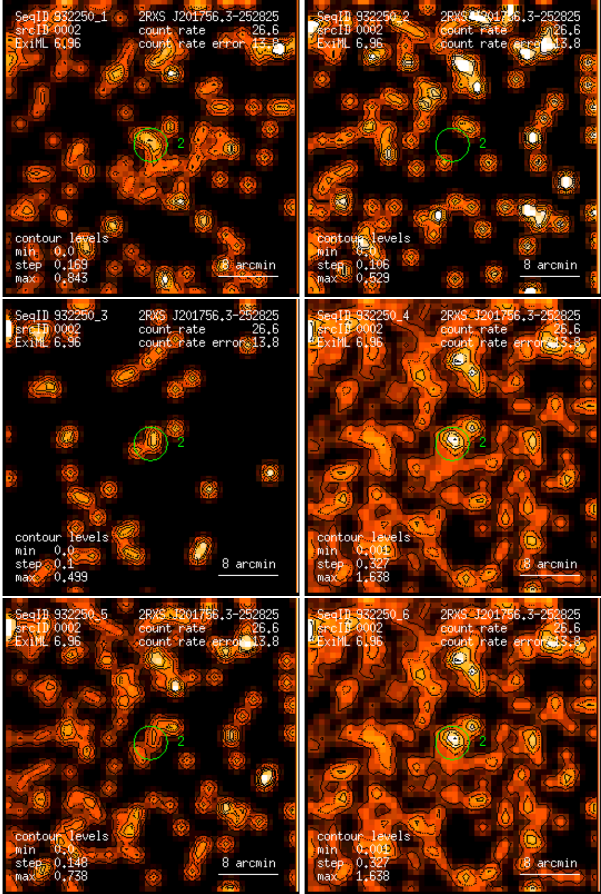
Figure 2: RASS 932250: detection 0002: band rate images, Gaussian filter: (1) PSPC channels 11 – 41, (2) 52 – 90, (3) 91 – 201, (4) 11 – 235, (5) 52 – 201, (6) 11 – 201. Broad band rates in counts/ks. Band rate contour levels in counts/ks/arcmin 2 .
