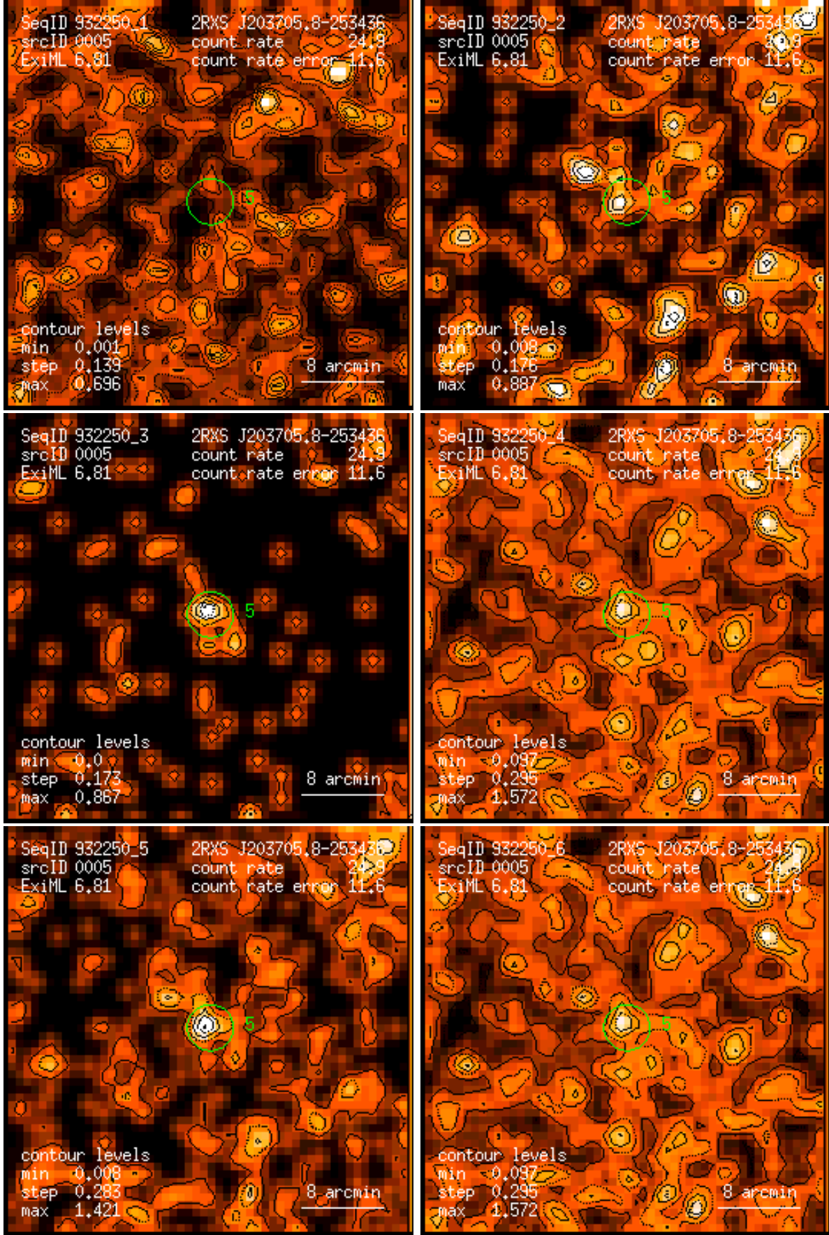
Figure 5: RASS 932250: detection 0005: band rate images, Gaussian filter: (1) PSPC channels 11 – 41, (2) 52 – 90, (3) 91 – 201, (4) 11 – 235, (5) 52 – 201, (6) 11 – 201. Broad band rates in counts/ks. Band rate contour levels in counts/ks/arcmin 2 .
