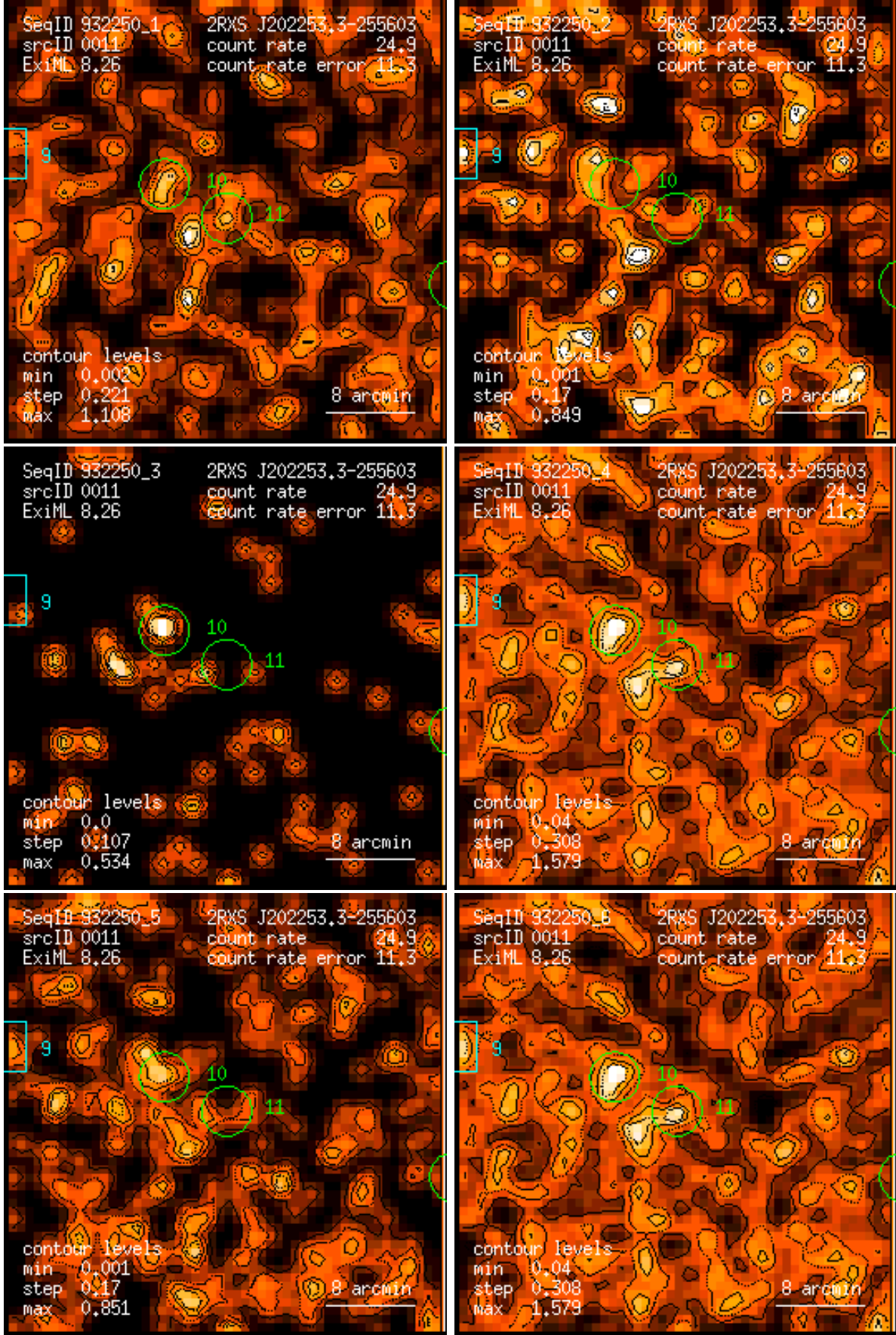
Figure 11: RASS 932250: detection 0011: band rate images, Gaussian filter: (1) PSPC channels 11 – 41, (2) 52 – 90, (3) 91 – 201, (4) 11 – 235, (5) 52 – 201, (6) 11 – 201. Broad band rates in counts/ks. Band rate contour levels in counts/ks/arcmin 2 .
