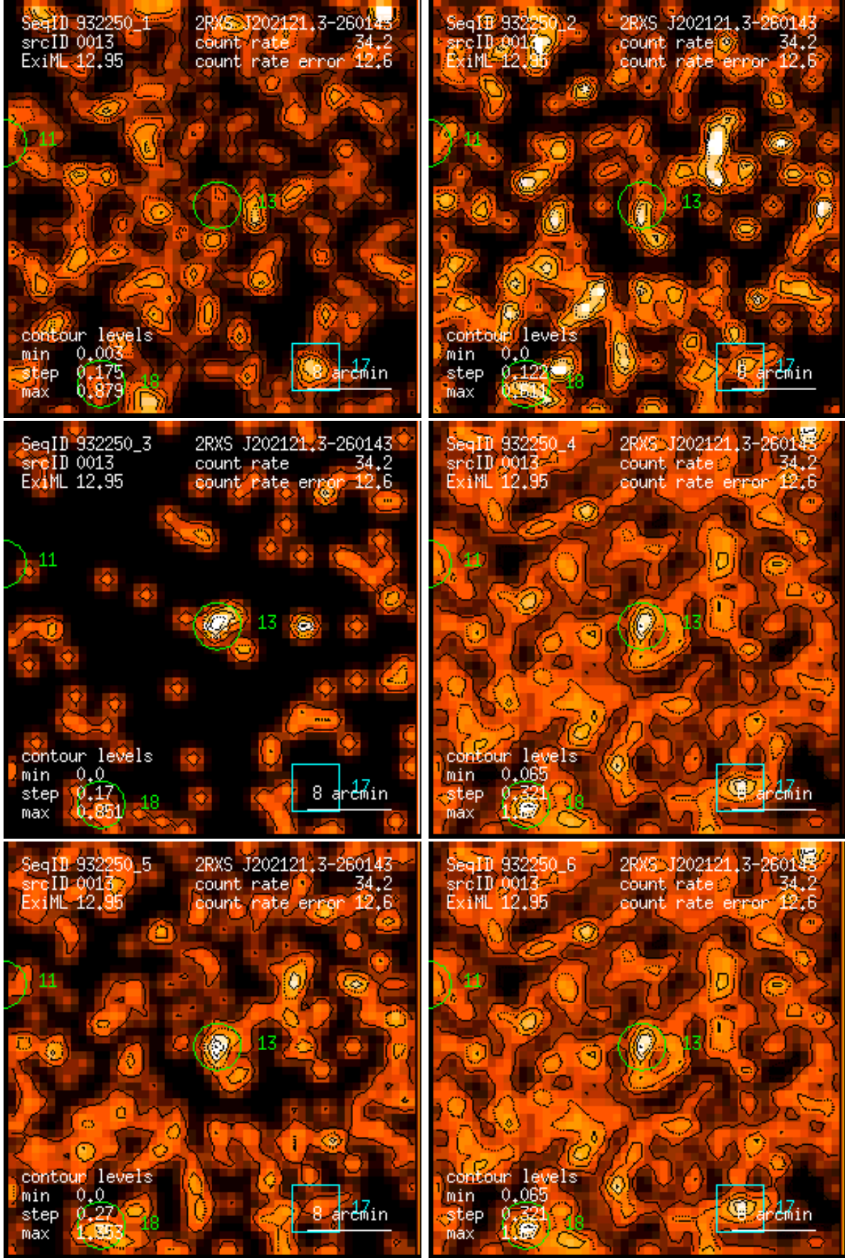
Figure 13: RASS 932250: detection 0013: band rate images, Gaussian filter: (1) PSPC channels 11 – 41, (2) 52 – 90, (3) 91 – 201, (4) 11 – 235, (5) 52 – 201, (6) 11 – 201. Broad band rates in counts/ks. Band rate contour levels in counts/ks/arcmin 2 .
