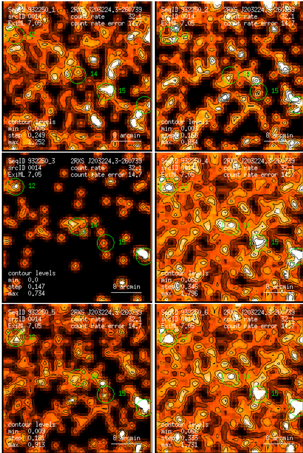
Figure 14: RASS 932250: detection 0014: band rate images, Gaussian filter: (1) PSPC channels 11 – 41, (2) 52 – 90, (3) 91 – 201, (4) 11 – 235, (5) 52 – 201, (6) 11 – 201. Broad band rates in counts/ks. Band rate contour levels in counts/ks/arcmin 2 .
