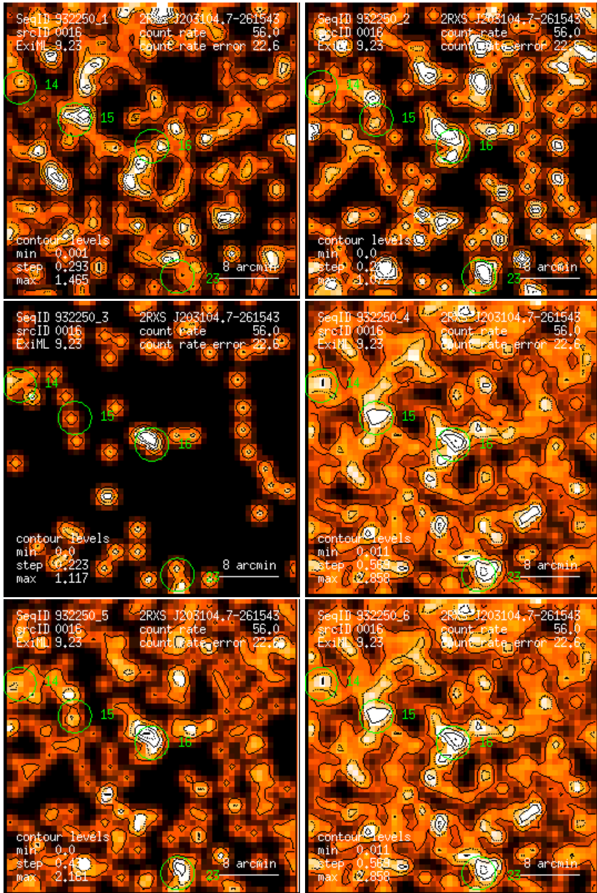
Figure 16: RASS 932250: detection 0016: band rate images, Gaussian filter: (1) PSPC channels 11 – 41, (2) 52 – 90, (3) 91 – 201, (4) 11 – 235, (5) 52 – 201, (6) 11 – 201. Broad band rates in counts/ks. Band rate contour levels in counts/ks/arcmin 2 .
