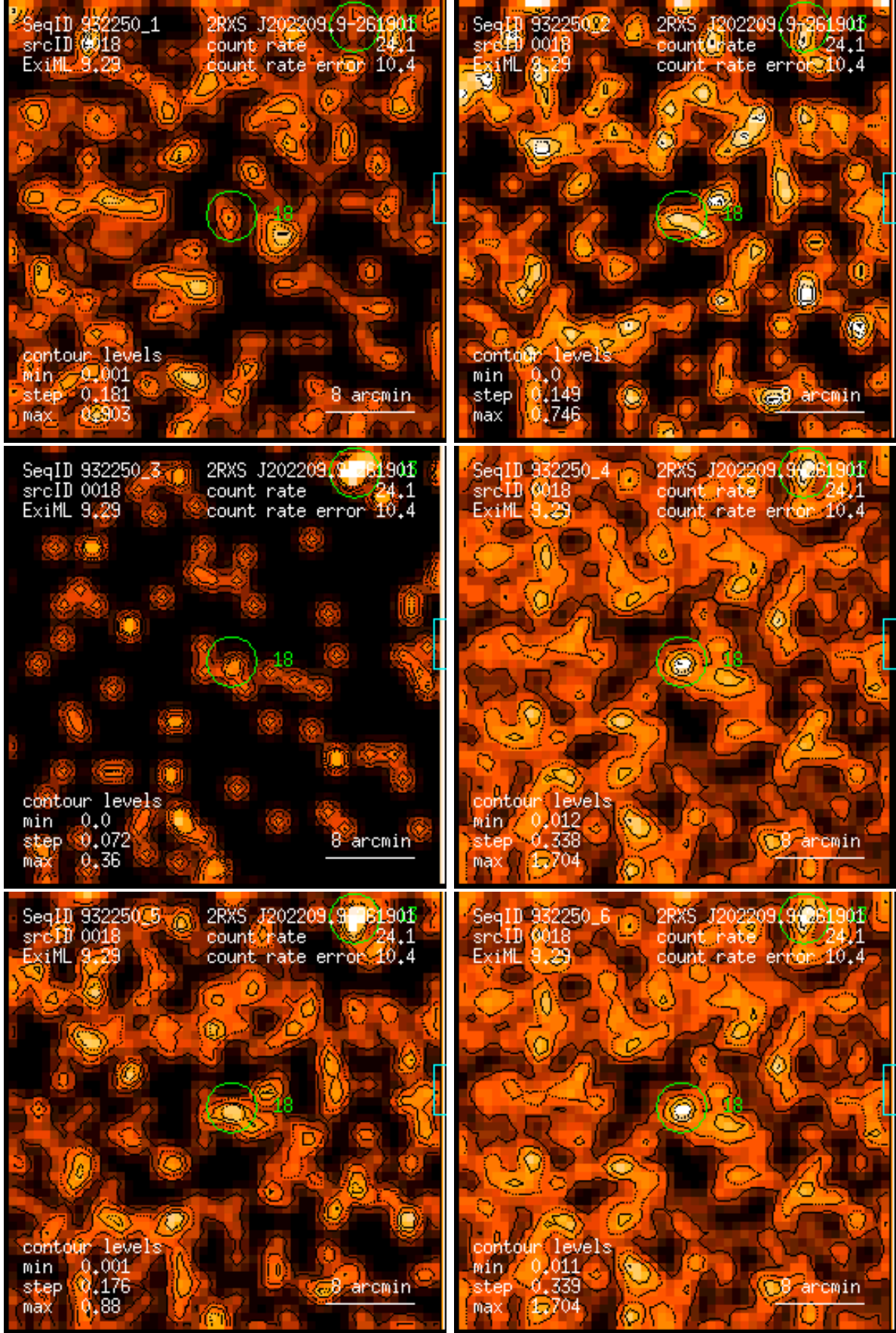
Figure 18: RASS 932250: detection 0018: band rate images, Gaussian filter: (1) PSPC channels 11 – 41, (2) 52 – 90, (3) 91 – 201, (4) 11 – 235, (5) 52 – 201, (6) 11 – 201. Broad band rates in counts/ks. Band rate contour levels in counts/ks/arcmin 2 .
