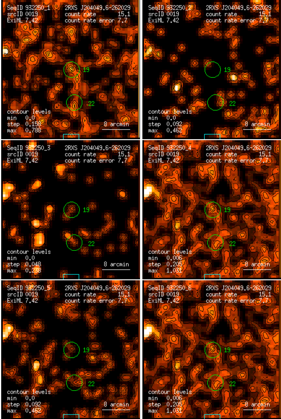
Figure 19: RASS 932250: detection 0019: band rate images, Gaussian filter: (1) PSPC channels 11 – 41, (2) 52 – 90, (3) 91 – 201, (4) 11 – 235, (5) 52 – 201, (6) 11 – 201. Broad band rates in counts/ks. Band rate contour levels in counts/ks/arcmin 2 .
