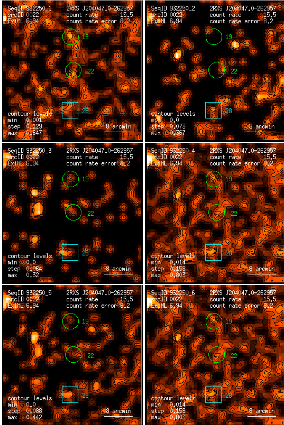
Figure 22: RASS 932250: detection 0022: band rate images, Gaussian filter: (1) PSPC channels 11 – 41, (2) 52 – 90, (3) 91 – 201, (4) 11 – 235, (5) 52 – 201, (6) 11 – 201. Broad band rates in counts/ks. Band rate contour levels in counts/ks/arcmin 2 .
