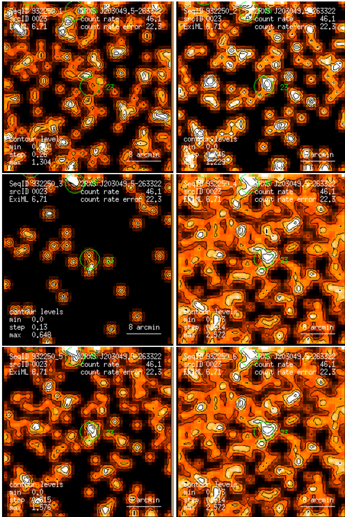
Figure 23: RASS 932250: detection 0023: band rate images, Gaussian filter: (1) PSPC channels 11 – 41, (2) 52 – 90, (3) 91 – 201, (4) 11 – 235, (5) 52 – 201, (6) 11 – 201. Broad band rates in counts/ks. Band rate contour levels in counts/ks/arcmin 2 .
