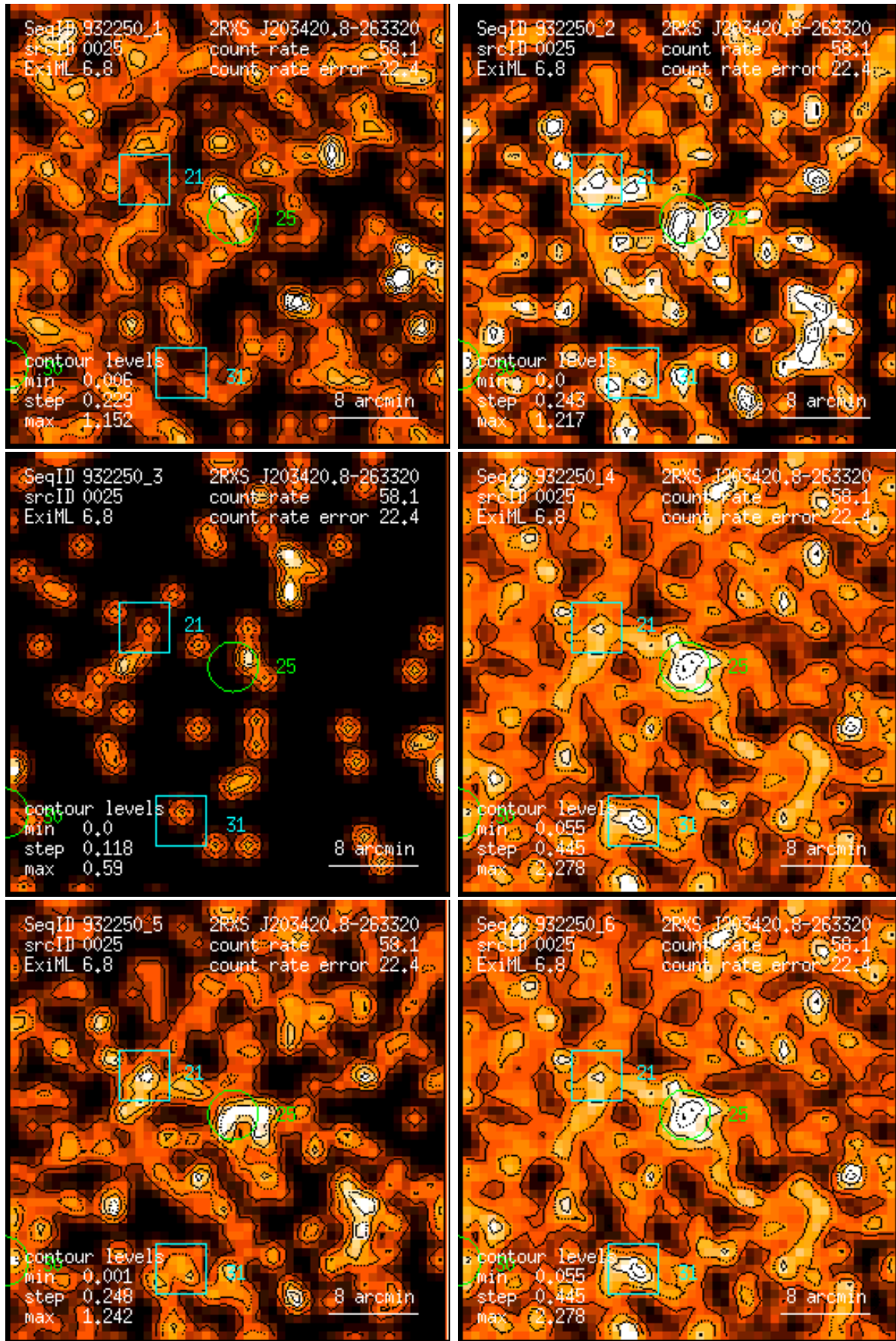
Figure 25: RASS 932250: detection 0025: band rate images, Gaussian filter: (1) PSPC channels 11 – 41, (2) 52 – 90, (3) 91 – 201, (4) 11 – 235, (5) 52 – 201, (6) 11 – 201. Broad band rates in counts/ks. Band rate contour levels in counts/ks/arcmin 2 .
