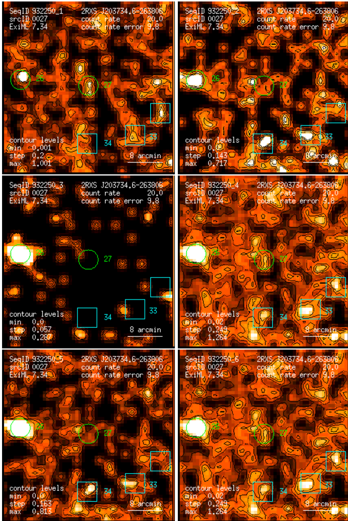
Figure 27: RASS 932250: detection 0027: band rate images, Gaussian filter: (1) PSPC channels 11 – 41, (2) 52 – 90, (3) 91 – 201, (4) 11 – 235, (5) 52 – 201, (6) 11 – 201. Broad band rates in counts/ks. Band rate contour levels in counts/ks/arcmin 2 .
