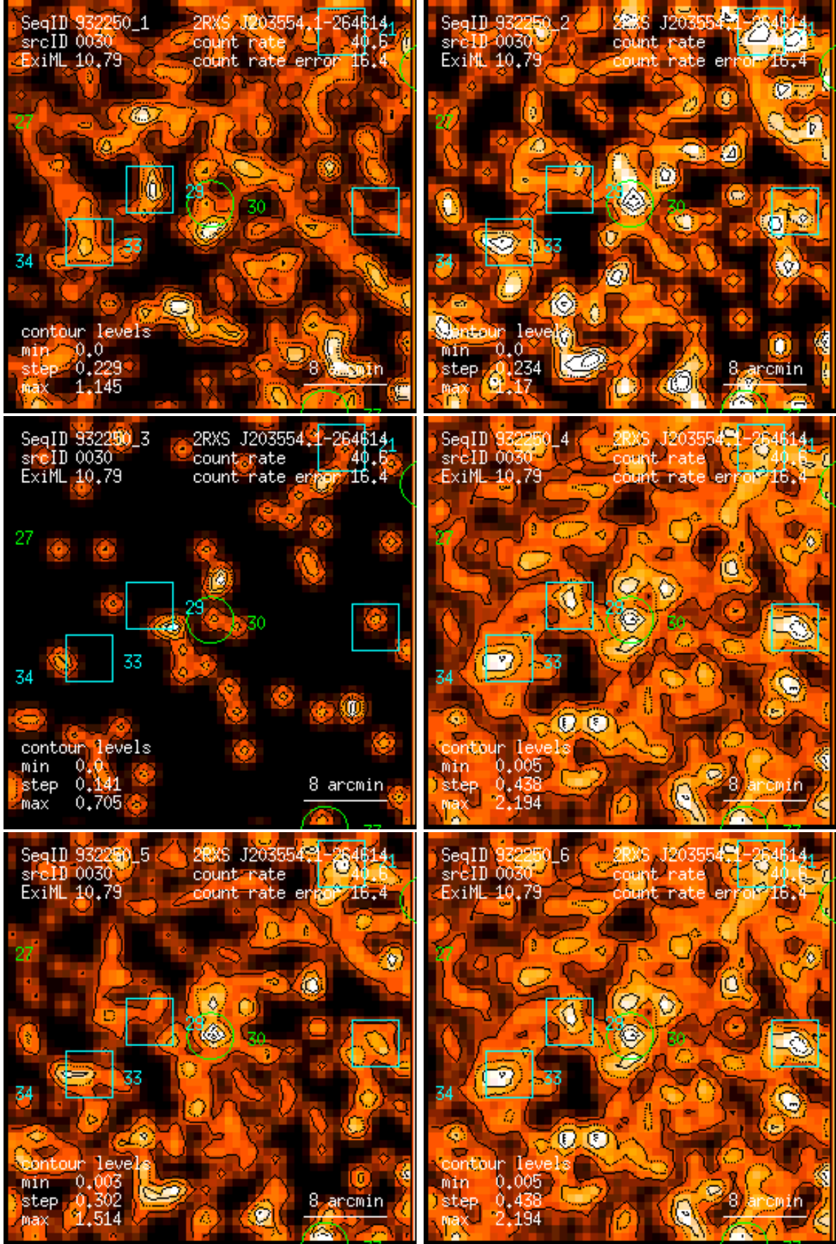
Figure 30: RASS 932250: detection 0030: band rate images, Gaussian filter: (1) PSPC channels 11 – 41, (2) 52 – 90, (3) 91 – 201, (4) 11 – 235, (5) 52 – 201, (6) 11 – 201. Broad band rates in counts/ks. Band rate contour levels in counts/ks/arcmin 2 .
