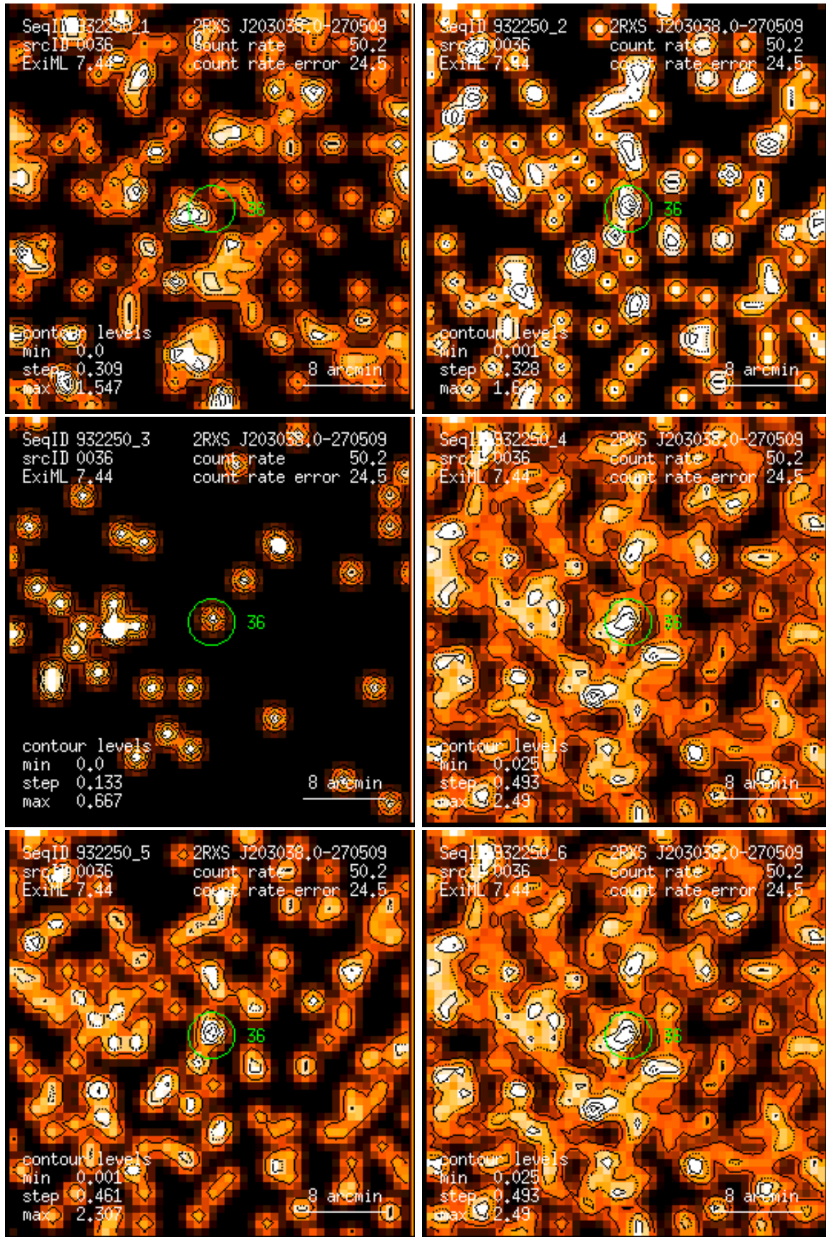
Figure 36: RASS 932250: detection 0036: band rate images, Gaussian filter: (1) PSPC channels 11 – 41, (2) 52 – 90, (3) 91 – 201, (4) 11 – 235, (5) 52 – 201, (6) 11 – 201. Broad band rates in counts/ks. Band rate contour levels in counts/ks/arcmin 2 .
