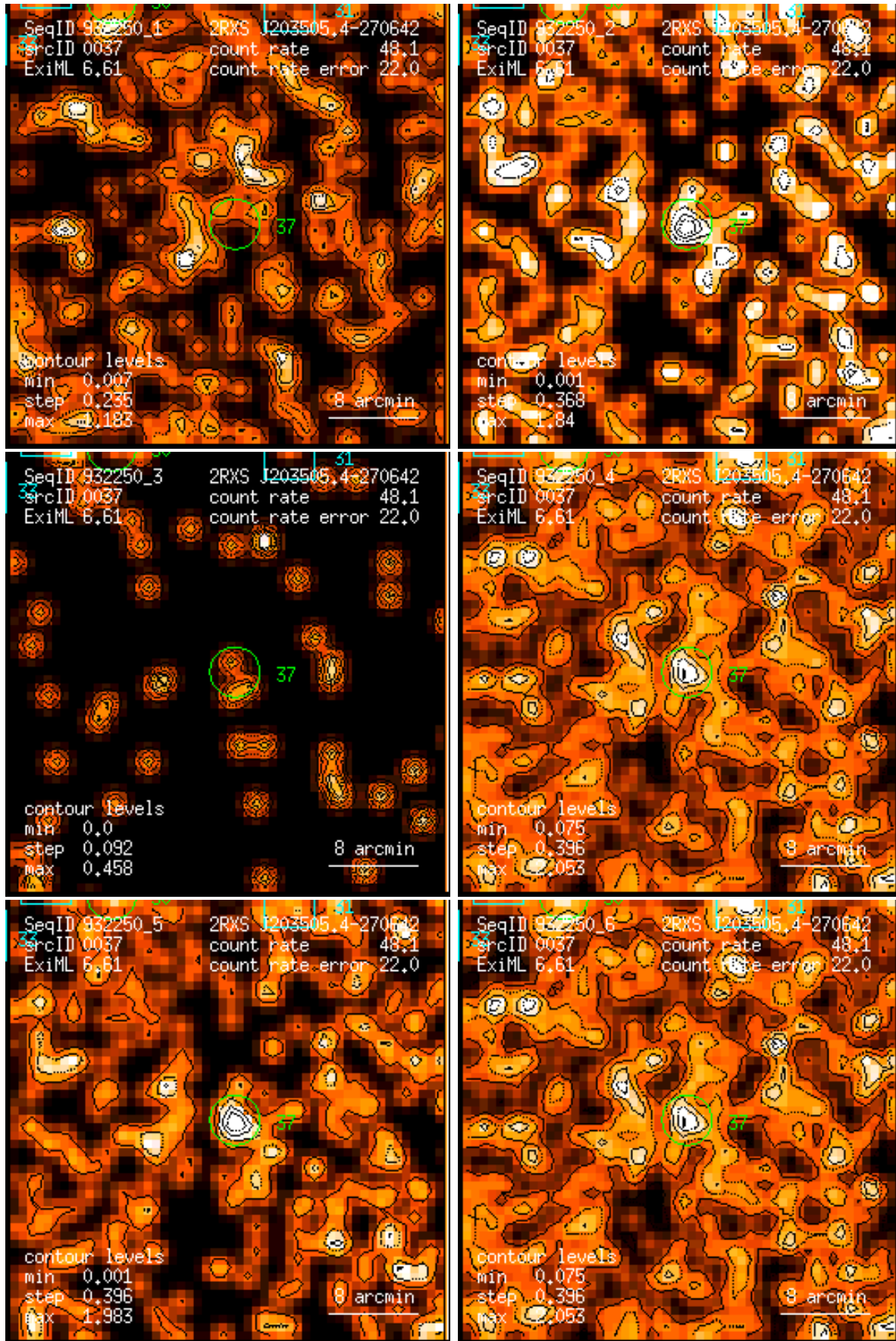
Figure 37: RASS 932250: detection 0037: band rate images, Gaussian filter: (1) PSPC channels 11 – 41, (2) 52 – 90, (3) 91 – 201, (4) 11 – 235, (5) 52 – 201, (6) 11 – 201. Broad band rates in counts/ks. Band rate contour levels in counts/ks/arcmin 2 .
