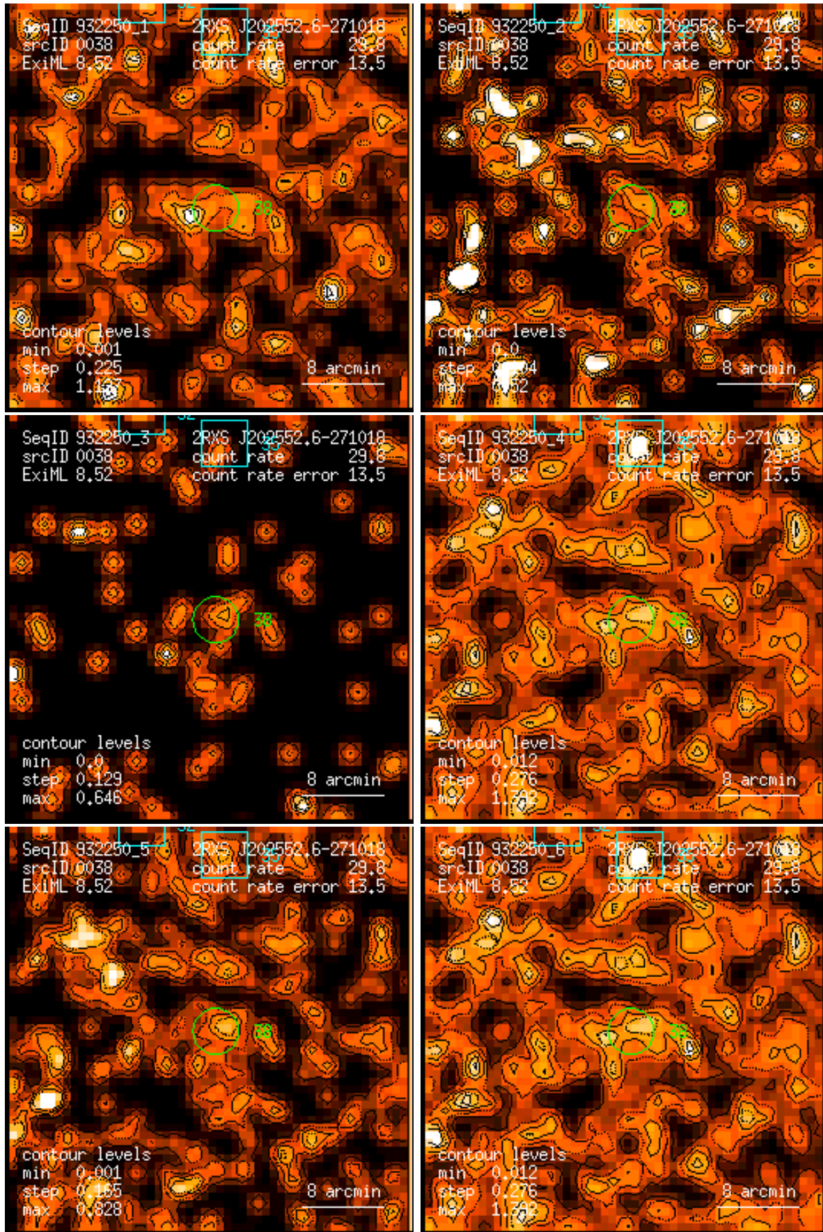
Figure 38: RASS 932250: detection 0038: band rate images, Gaussian filter: (1) PSPC channels 11 – 41, (2) 52 – 90, (3) 91 – 201, (4) 11 – 235, (5) 52 – 201, (6) 11 – 201. Broad band rates in counts/ks. Band rate contour levels in counts/ks/arcmin 2 .
