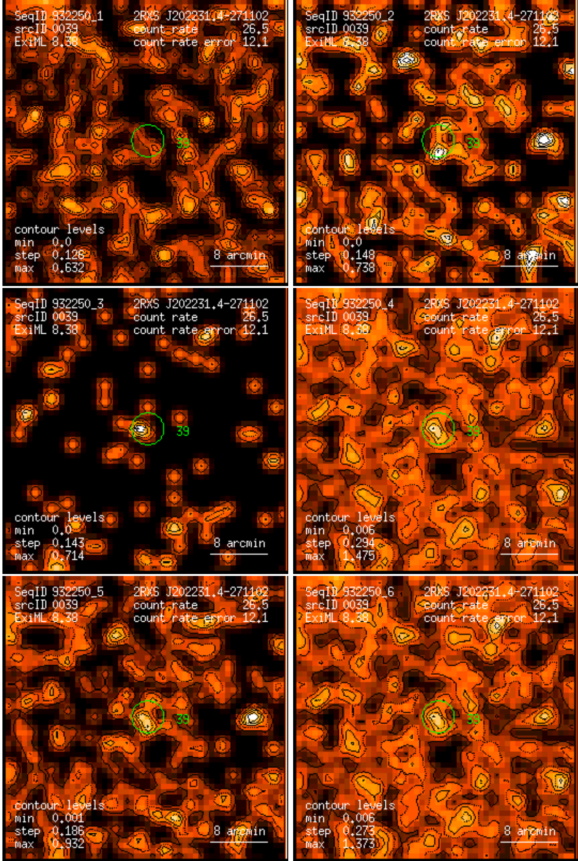
Figure 39: RASS 932250: detection 0039: band rate images, Gaussian filter: (1) PSPC channels 11 – 41, (2) 52 – 90, (3) 91 – 201, (4) 11 – 235, (5) 52 – 201, (6) 11 – 201. Broad band rates in counts/ks. Band rate contour levels in counts/ks/arcmin 2 .
