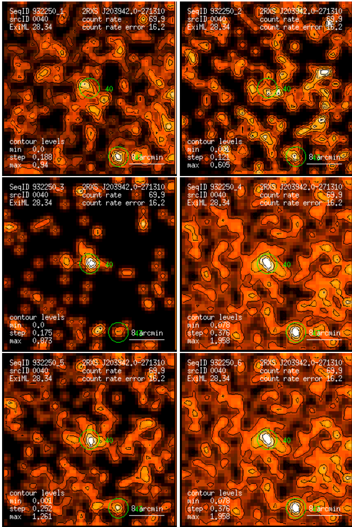
Figure 40: RASS 932250: detection 0040: band rate images, Gaussian filter: (1) PSPC channels 11 – 41, (2) 52 – 90, (3) 91 – 201, (4) 11 – 235, (5) 52 – 201, (6) 11 – 201. Broad band rates in counts/ks. Band rate contour levels in counts/ks/arcmin 2 .
