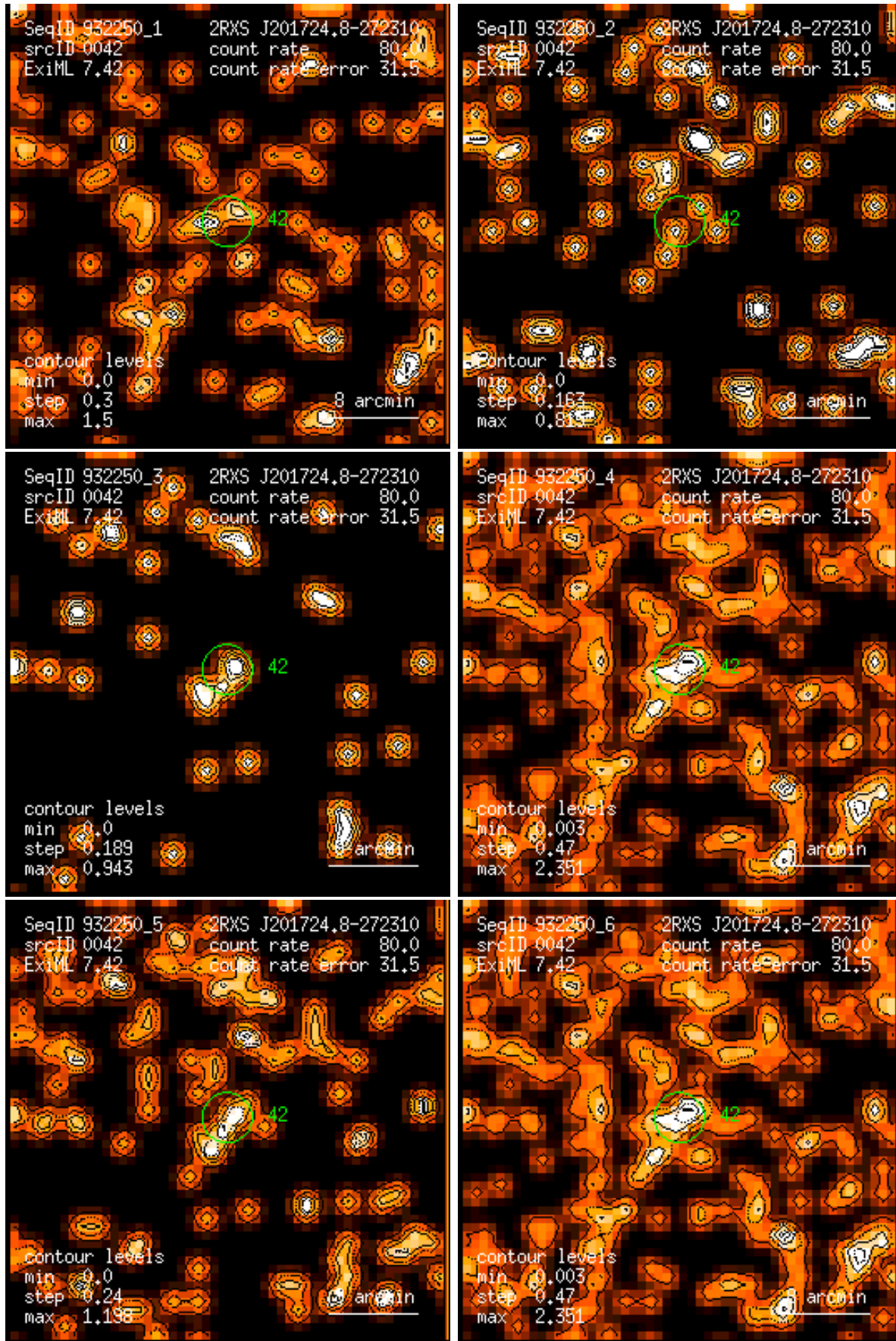
Figure 42: RASS 932250: detection 0042: band rate images, Gaussian filter: (1) PSPC channels 11 – 41, (2) 52 – 90, (3) 91 – 201, (4) 11 – 235, (5) 52 – 201, (6) 11 – 201. Broad band rates in counts/ks. Band rate contour levels in counts/ks/arcmin 2 .
