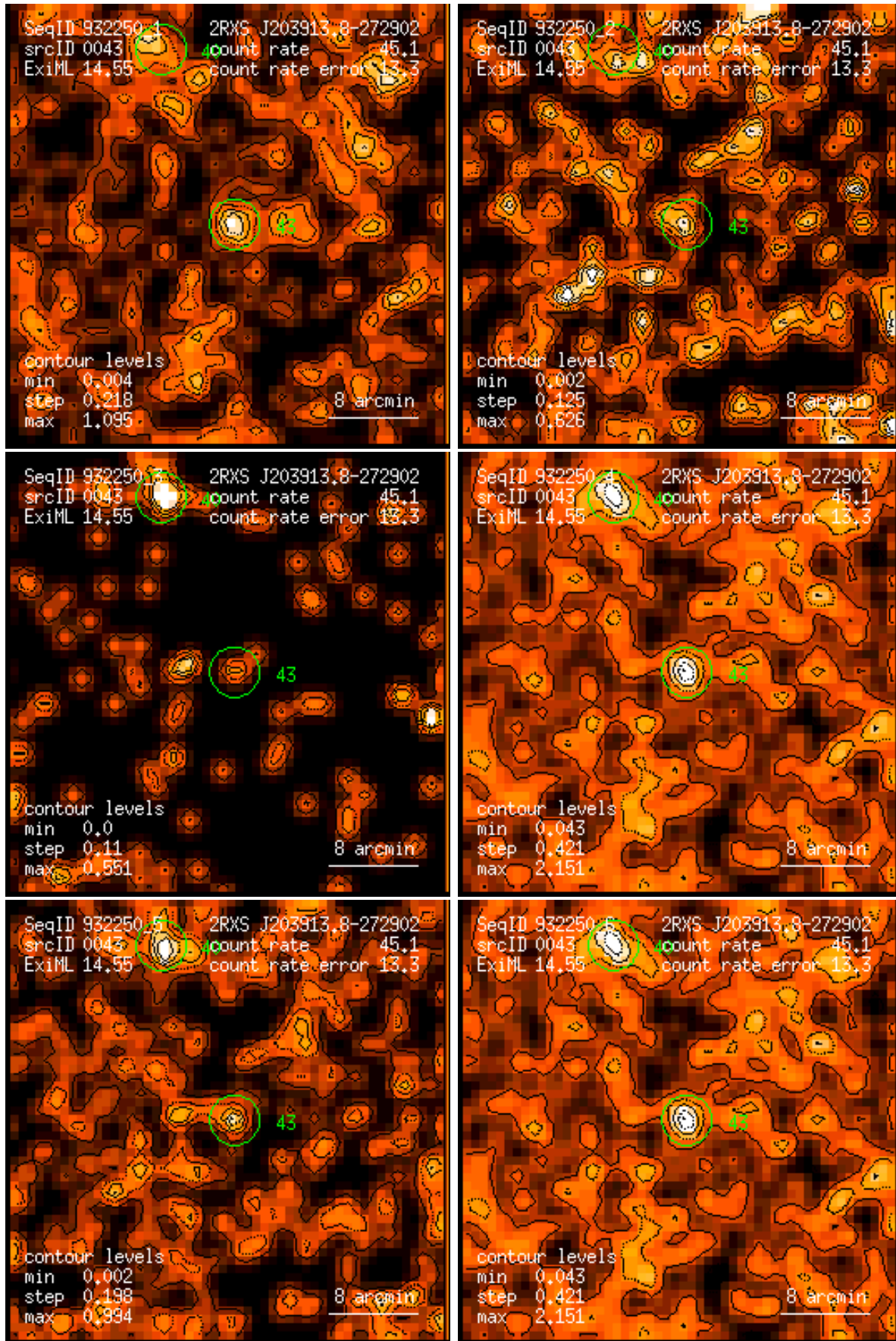
Figure 43: RASS 932250: detection 0043: band rate images, Gaussian filter: (1) PSPC channels 11 – 41, (2) 52 – 90, (3) 91 – 201, (4) 11 – 235, (5) 52 – 201, (6) 11 – 201. Broad band rates in counts/ks. Band rate contour levels in counts/ks/arcmin 2 .
