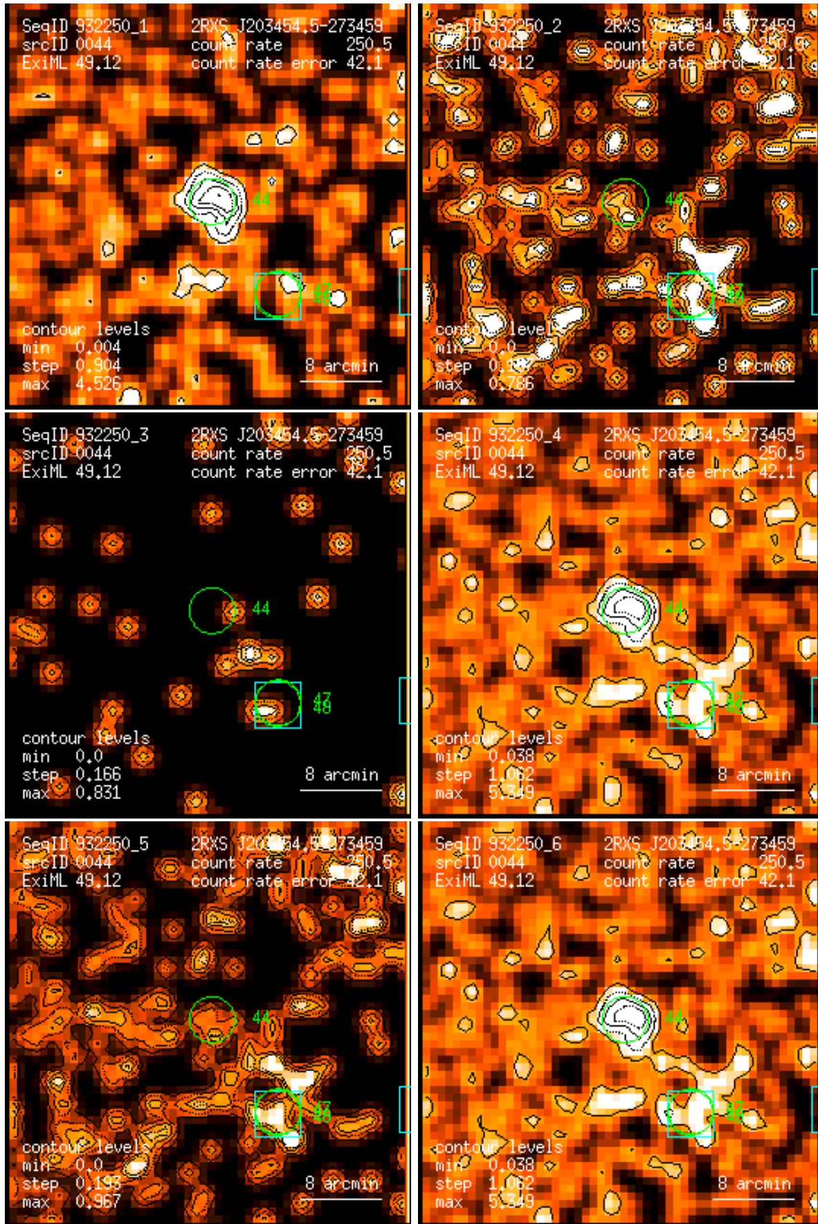
Figure 44: RASS 932250: detection 0044: band rate images, Gaussian filter: (1) PSPC channels 11 – 41, (2) 52 – 90, (3) 91 – 201, (4) 11 – 235, (5) 52 – 201, (6) 11 – 201. Broad band rates in counts/ks. Band rate contour levels in counts/ks/arcmin 2 .
