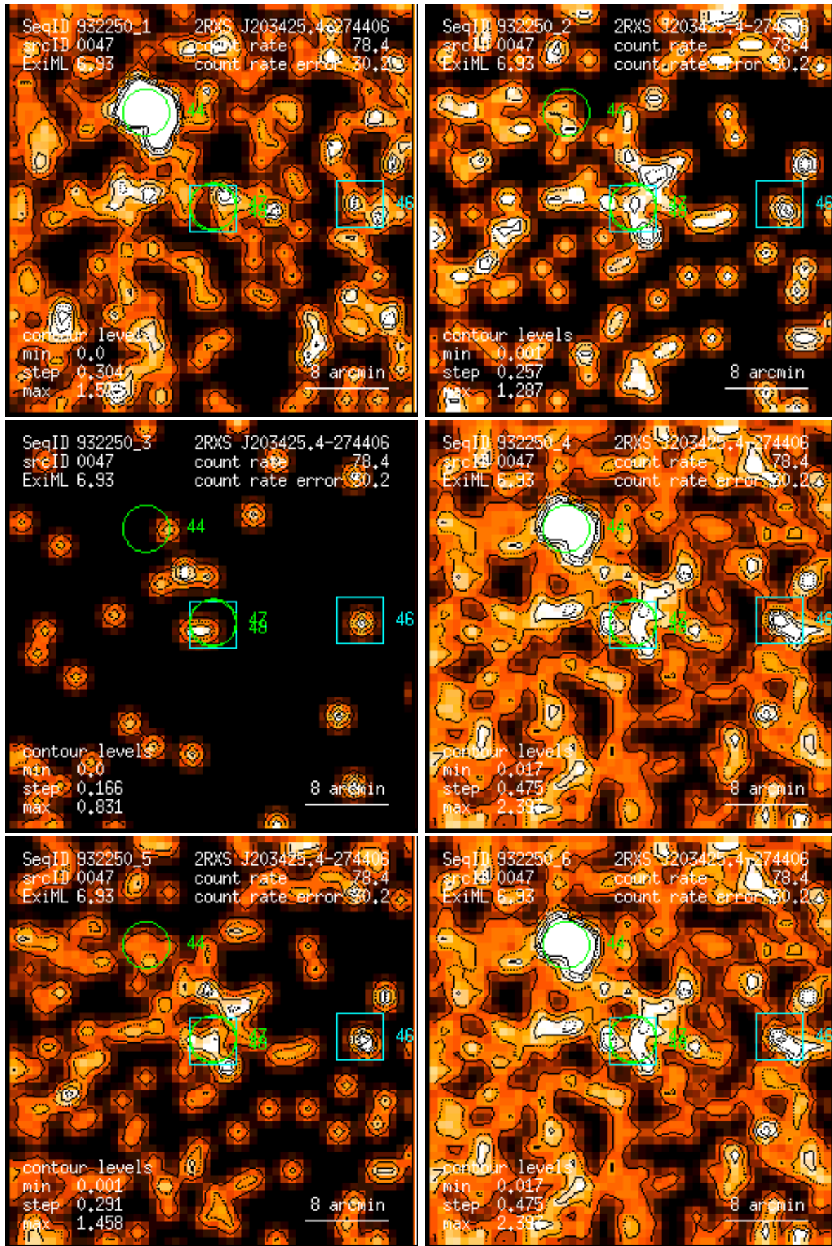
Figure 47: RASS 932250: detection 0047: band rate images, Gaussian filter: (1) PSPC channels 11 – 41, (2) 52 – 90, (3) 91 – 201, (4) 11 – 235, (5) 52 – 201, (6) 11 – 201. Broad band rates in counts/ks. Band rate contour levels in counts/ks/arcmin 2 .
