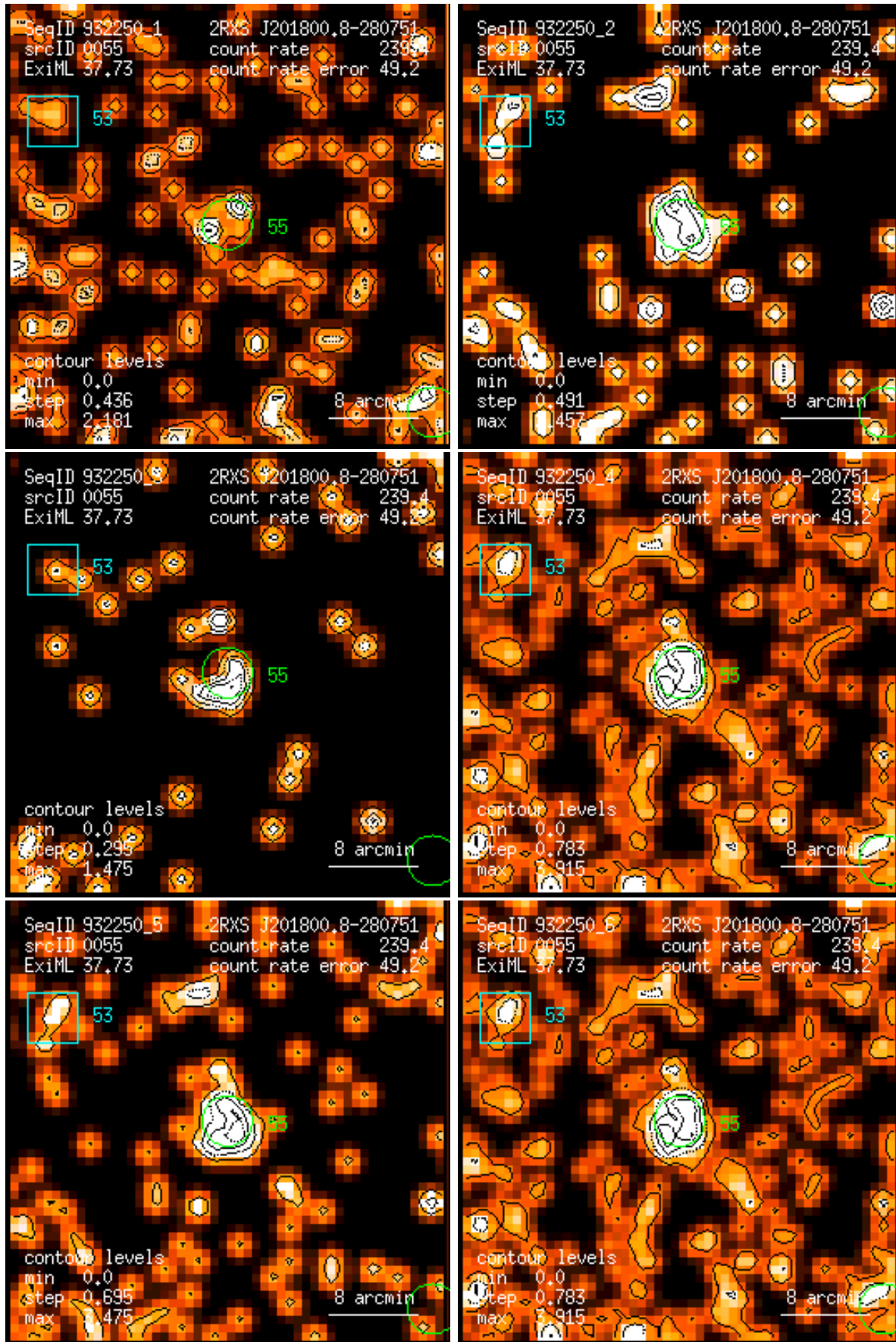
Figure 55: RASS 932250: detection 0055: band rate images, Gaussian filter: (1) PSPC channels 11 – 41, (2) 52 – 90, (3) 91 – 201, (4) 11 – 235, (5) 52 – 201, (6) 11 – 201. Broad band rates in counts/ks. Band rate contour levels in counts/ks/arcmin 2 .
