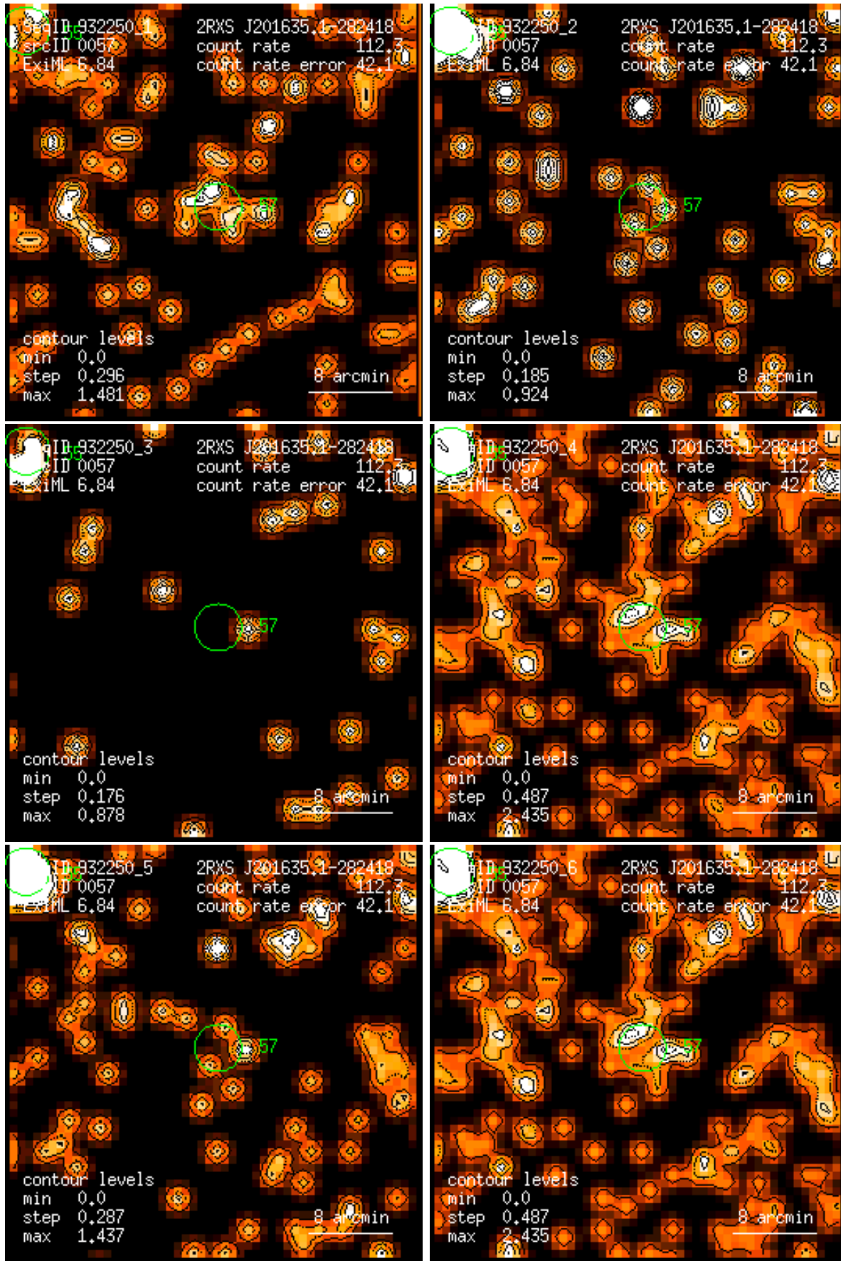
Figure 57: RASS 932250: detection 0057: band rate images, Gaussian filter: (1) PSPC channels 11 – 41, (2) 52 – 90, (3) 91 – 201, (4) 11 – 235, (5) 52 – 201, (6) 11 – 201. Broad band rates in counts/ks. Band rate contour levels in counts/ks/arcmin 2 .
