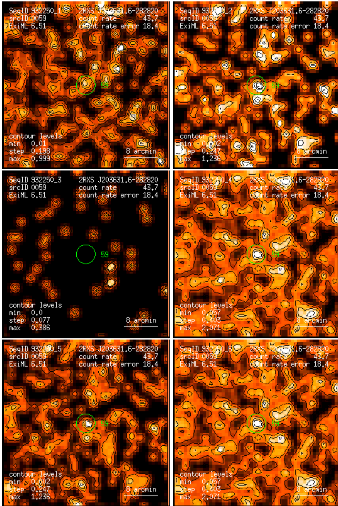
Figure 59: RASS 932250: detection 0059: band rate images, Gaussian filter: (1) PSPC channels 11 – 41, (2) 52 – 90, (3) 91 – 201, (4) 11 – 235, (5) 52 – 201, (6) 11 – 201. Broad band rates in counts/ks. Band rate contour levels in counts/ks/arcmin 2 .
