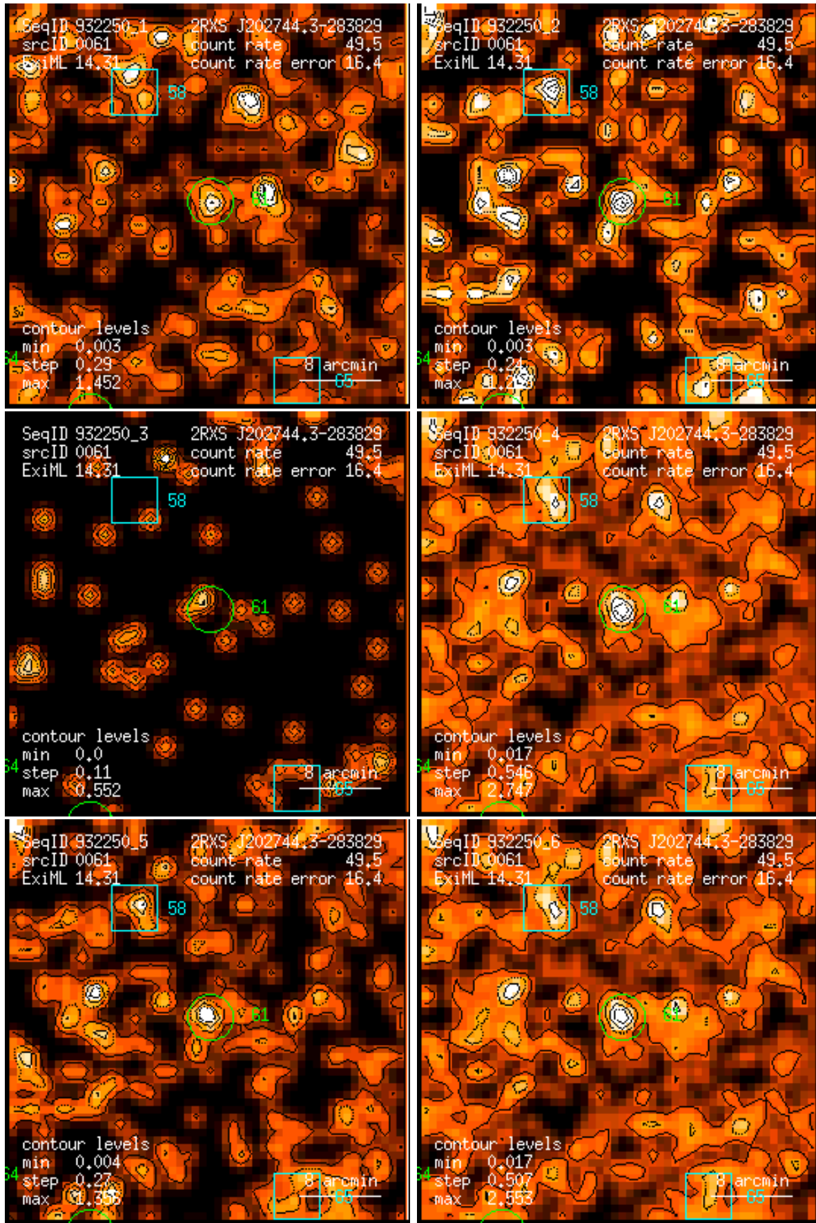
Figure 61: RASS 932250: detection 0061: band rate images, Gaussian filter: (1) PSPC channels 11 – 41, (2) 52 – 90, (3) 91 – 201, (4) 11 – 235, (5) 52 – 201, (6) 11 – 201. Broad band rates in counts/ks. Band rate contour levels in counts/ks/arcmin 2 .
