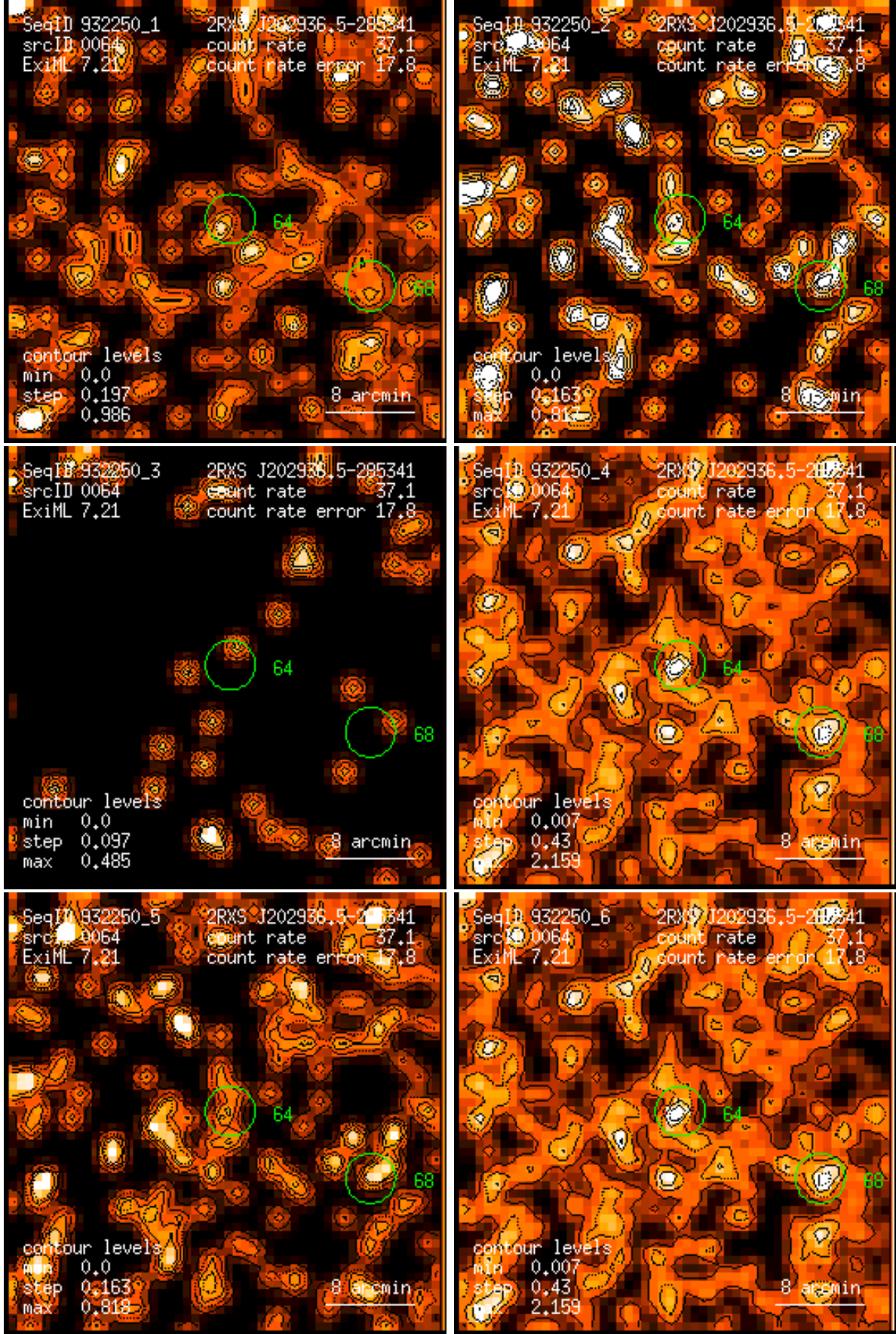
Figure 64: RASS 932250: detection 0064: band rate images, Gaussian filter: (1) PSPC channels 11 – 41, (2) 52 – 90, (3) 91 – 201, (4) 11 – 235, (5) 52 – 201, (6) 11 – 201. Broad band rates in counts/ks. Band rate contour levels in counts/ks/arcmin 2 .
