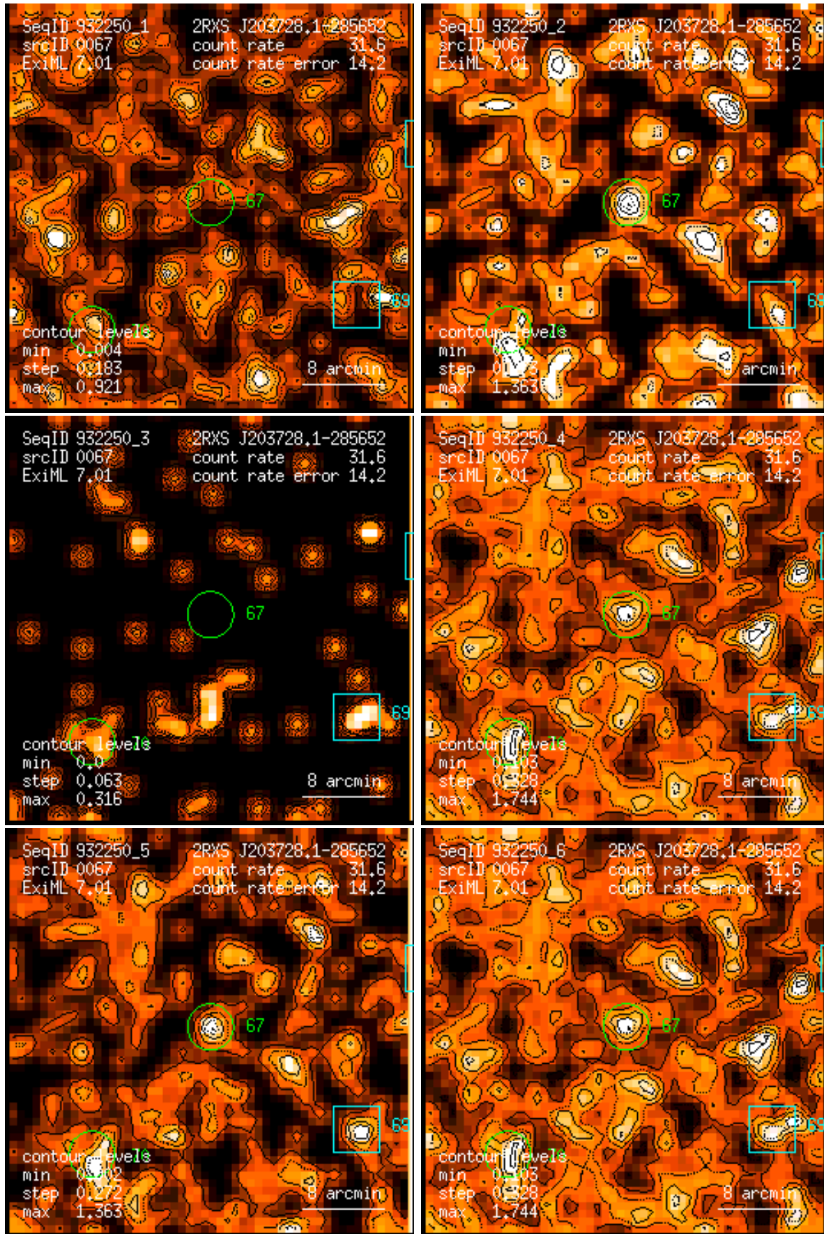
Figure 67: RASS 932250: detection 0067: band rate images, Gaussian filter: (1) PSPC channels 11 – 41, (2) 52 – 90, (3) 91 – 201, (4) 11 – 235, (5) 52 – 201, (6) 11 – 201. Broad band rates in counts/ks. Band rate contour levels in counts/ks/arcmin 2 .
