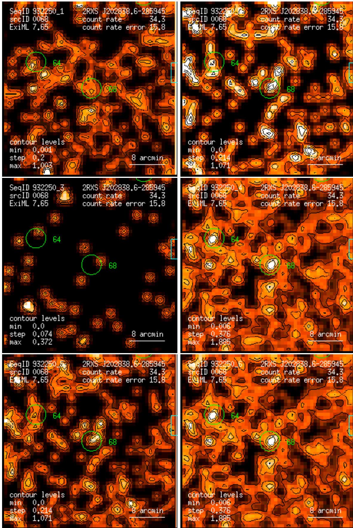
Figure 68: RASS 932250: detection 0068: band rate images, Gaussian filter: (1) PSPC channels 11 – 41, (2) 52 – 90, (3) 91 – 201, (4) 11 – 235, (5) 52 – 201, (6) 11 – 201. Broad band rates in counts/ks. Band rate contour levels in counts/ks/arcmin 2 .
